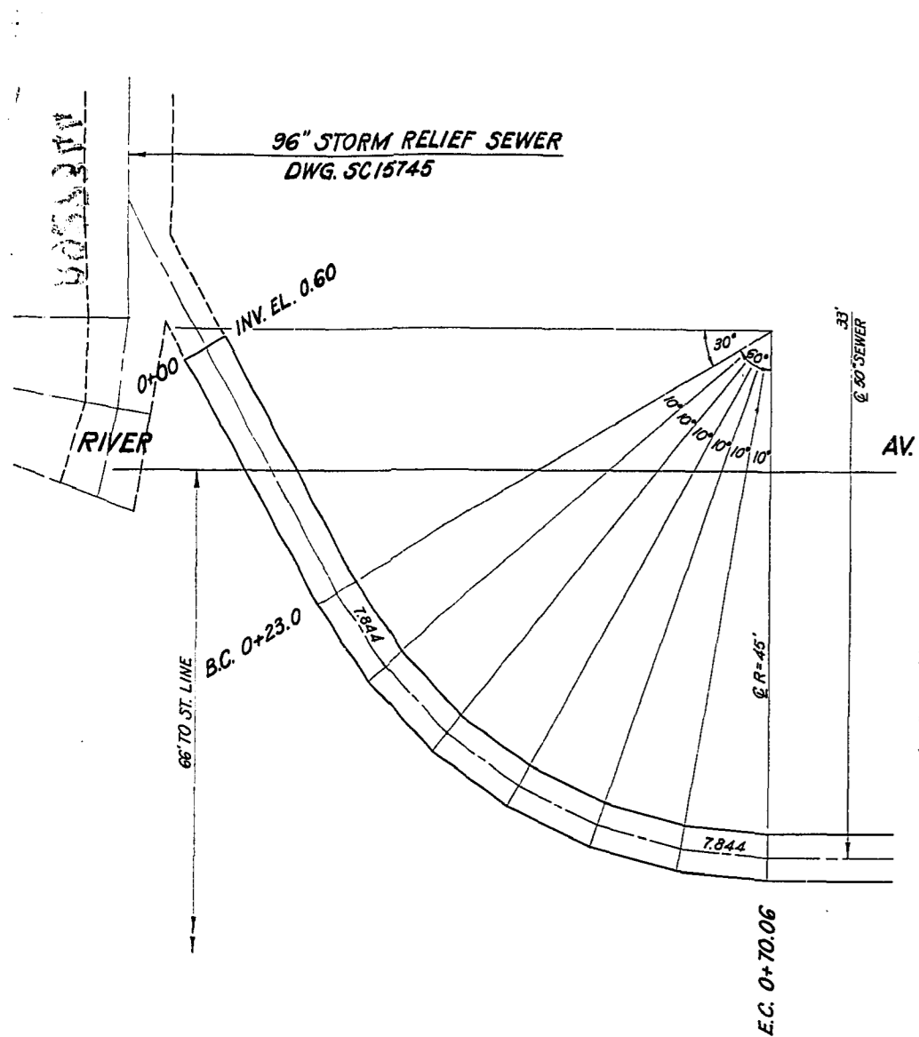
DETAIL OF \frac{1}{2} OF SEWER @ RIVER AV. AND FORT ROUGE PARK
