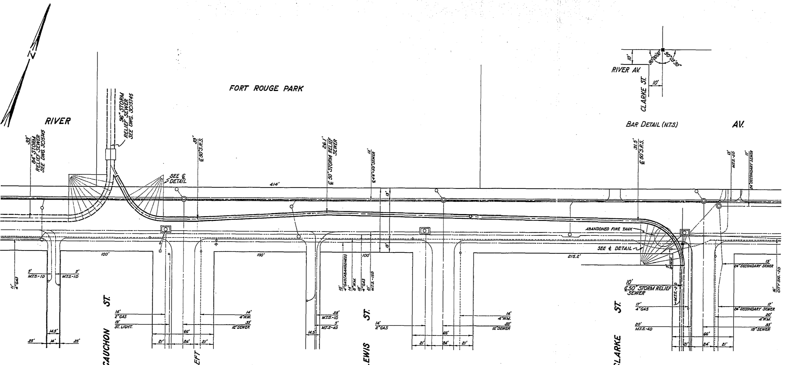
DETAIL OF \frac{1}{2} OF SEWER @ RIVER AV. AND FORT ROUGE PARK
