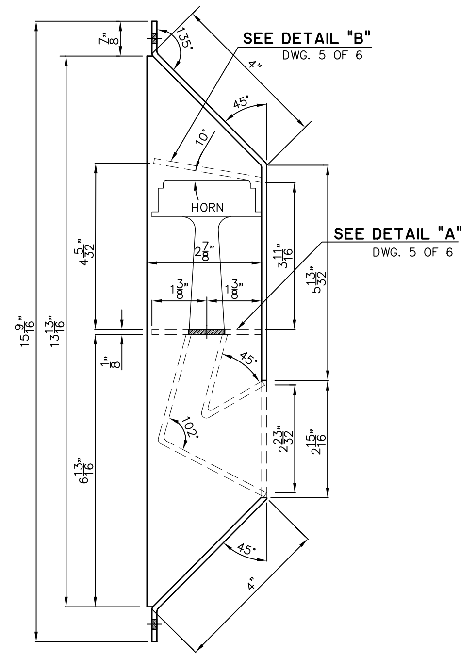
SIDE VIEW
