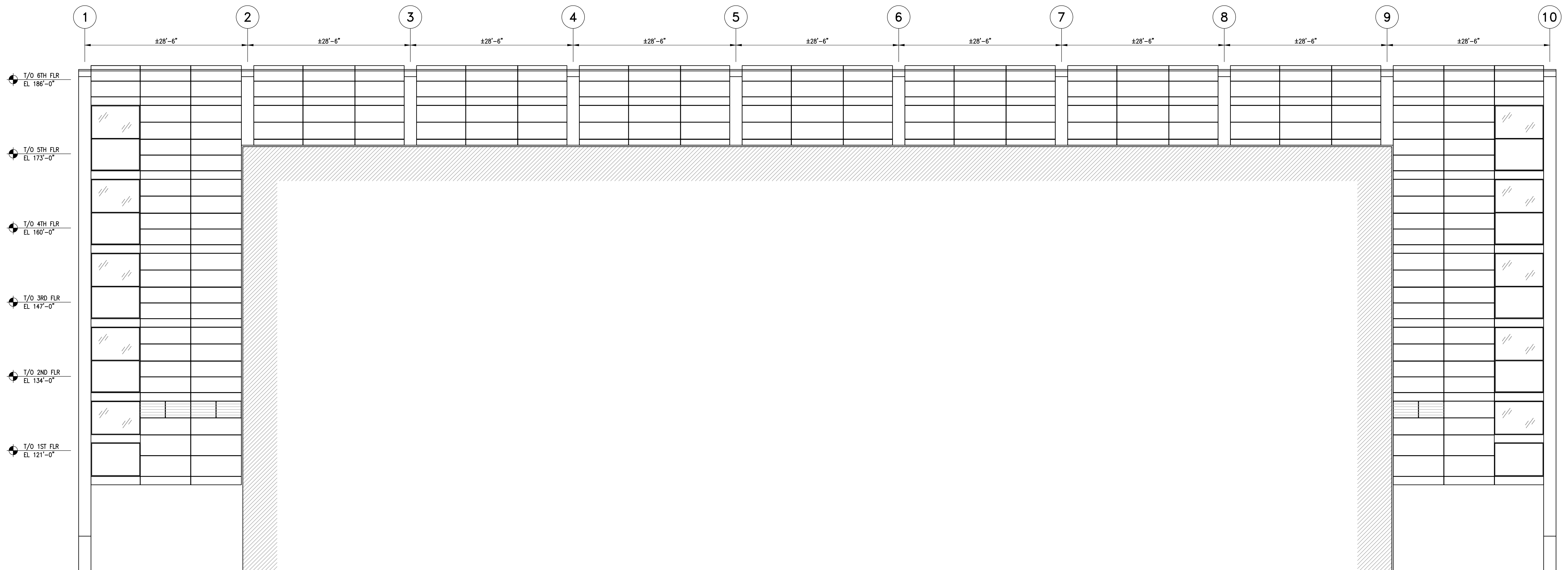
1 SOUTH ELEVATION S1.5 1/8" = 1'-0"
