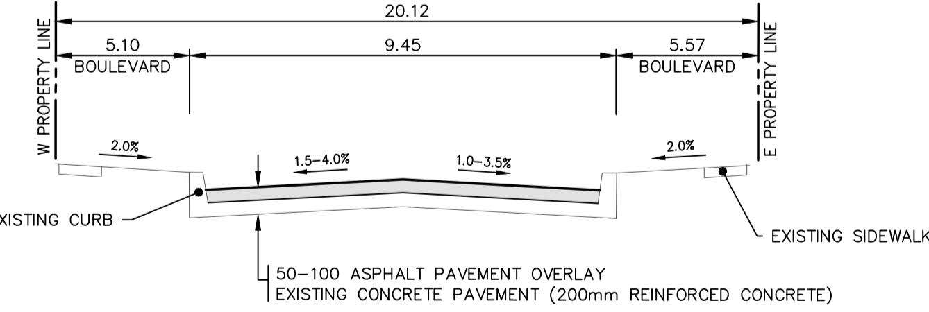
TYPICAL CROSS-SECTION NTS
