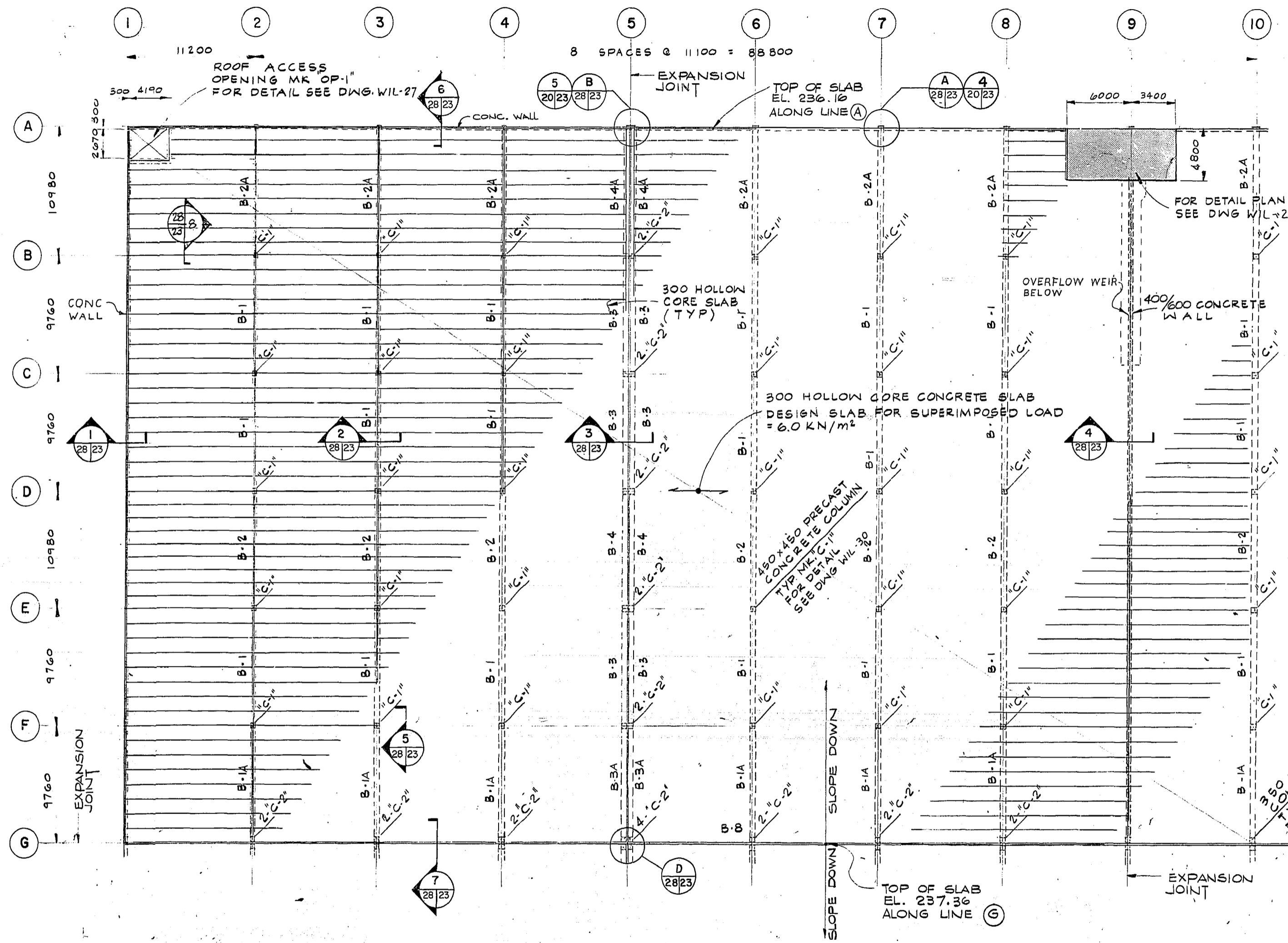
ROOF PLAN AREA 'A'
