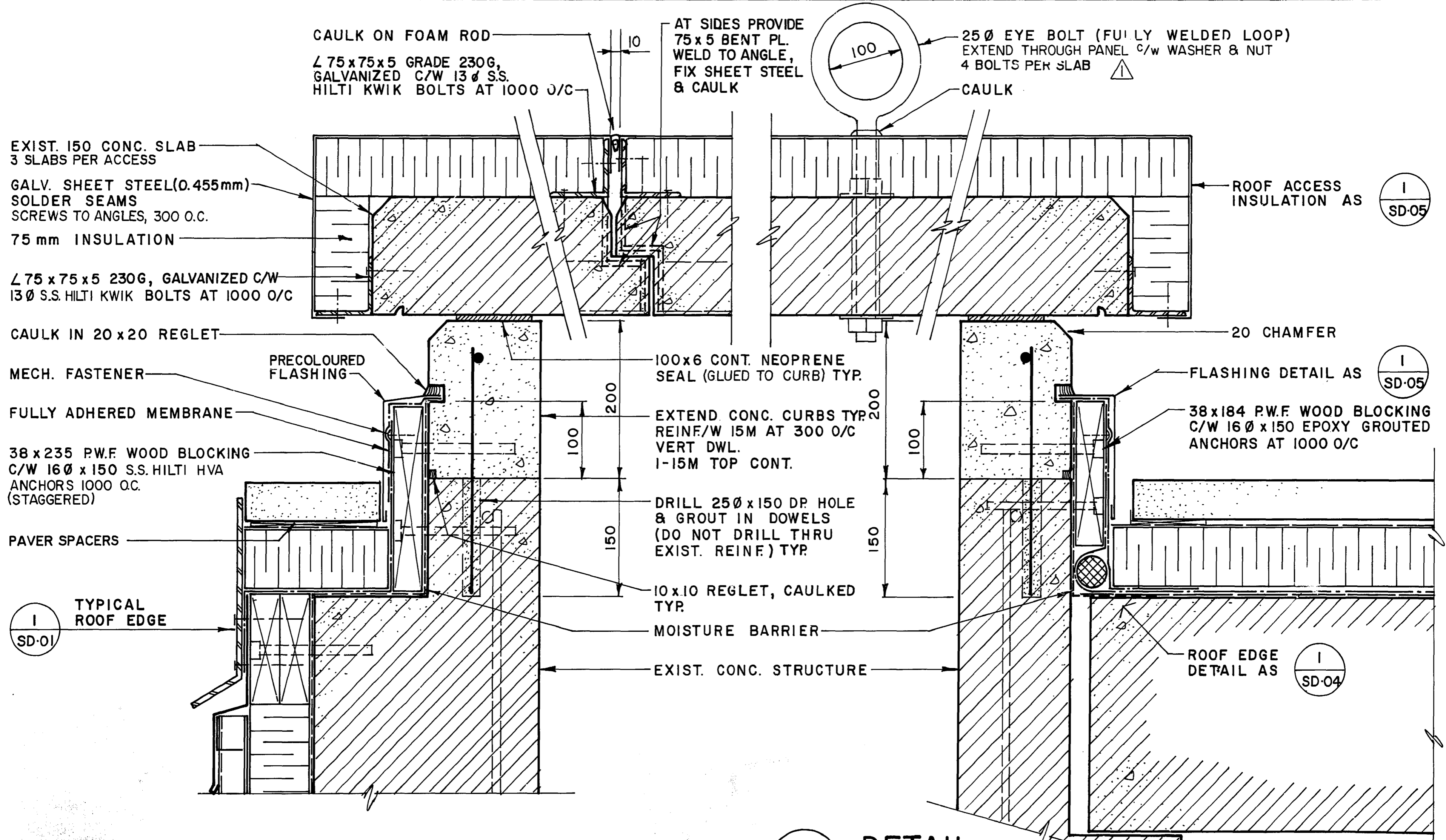
1 SD-05 DETAIL 1:5
