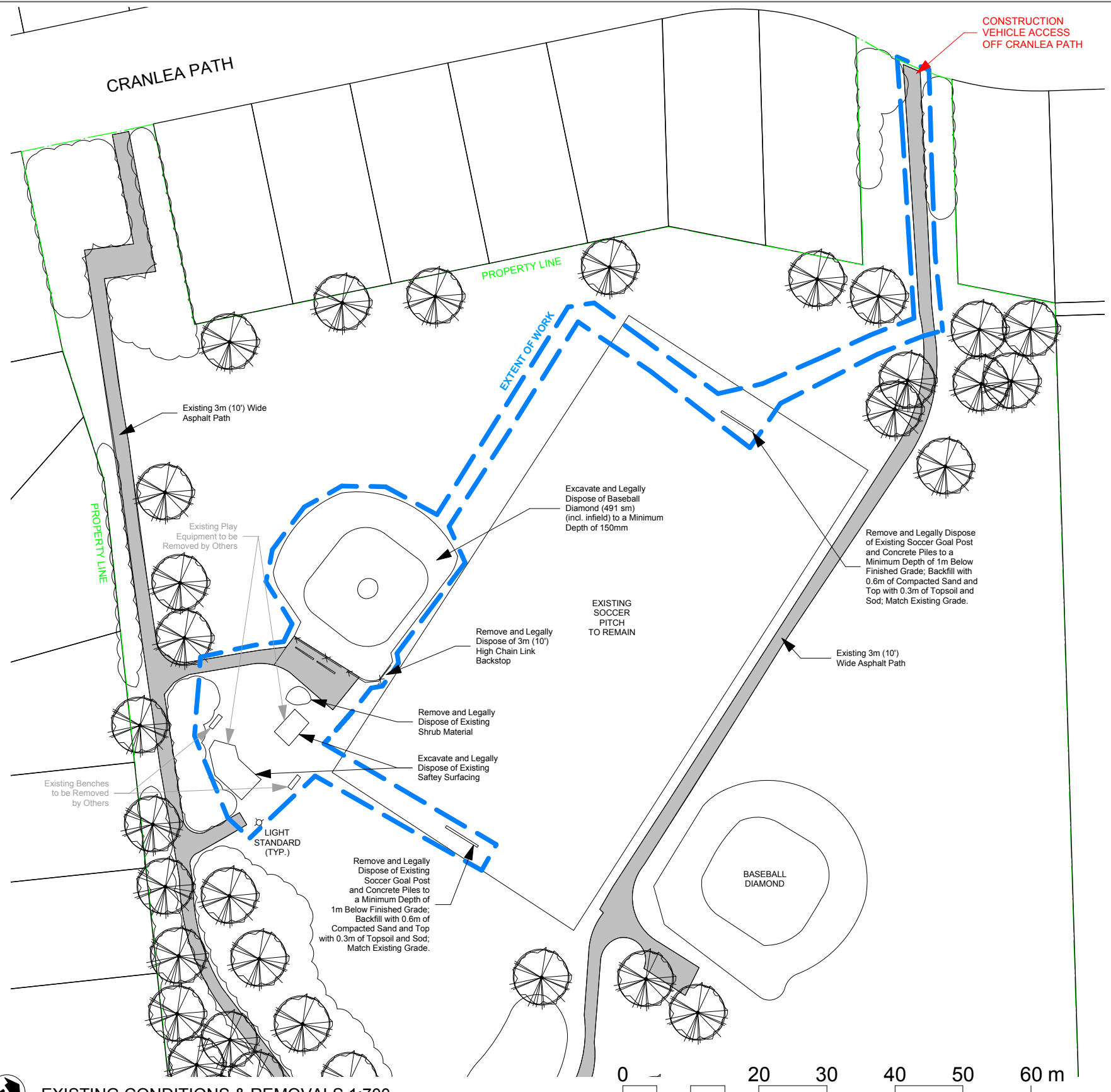
EXISTING CONDITIONS & REMOVALS 1:700
