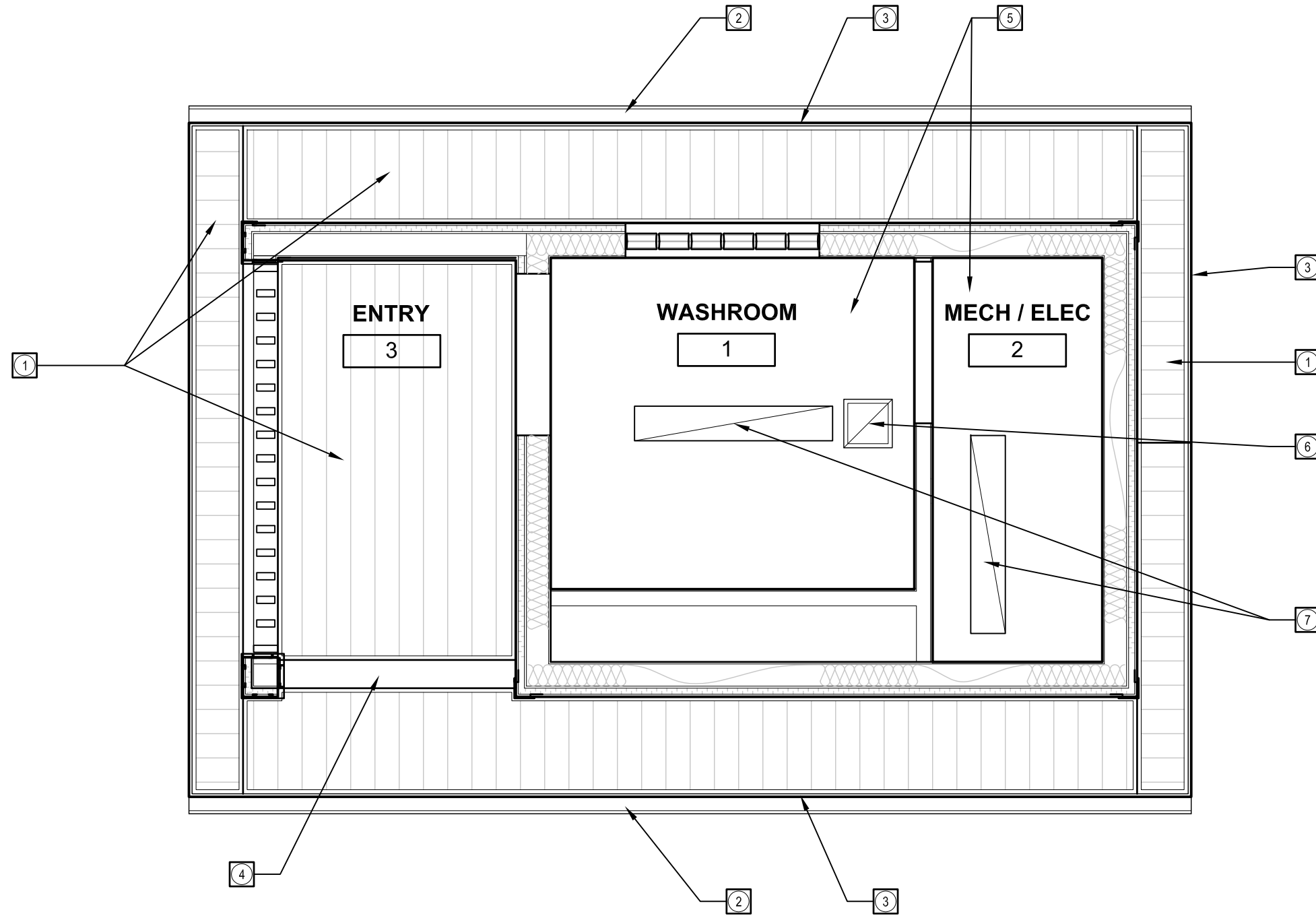
1 A-3 REFLECTED CEILING PLAN SCALE 3/8" = 1'-0"
