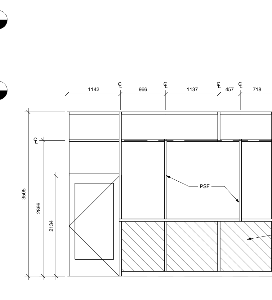
8 CURTAIN PANEL INTERIOR 1:50
