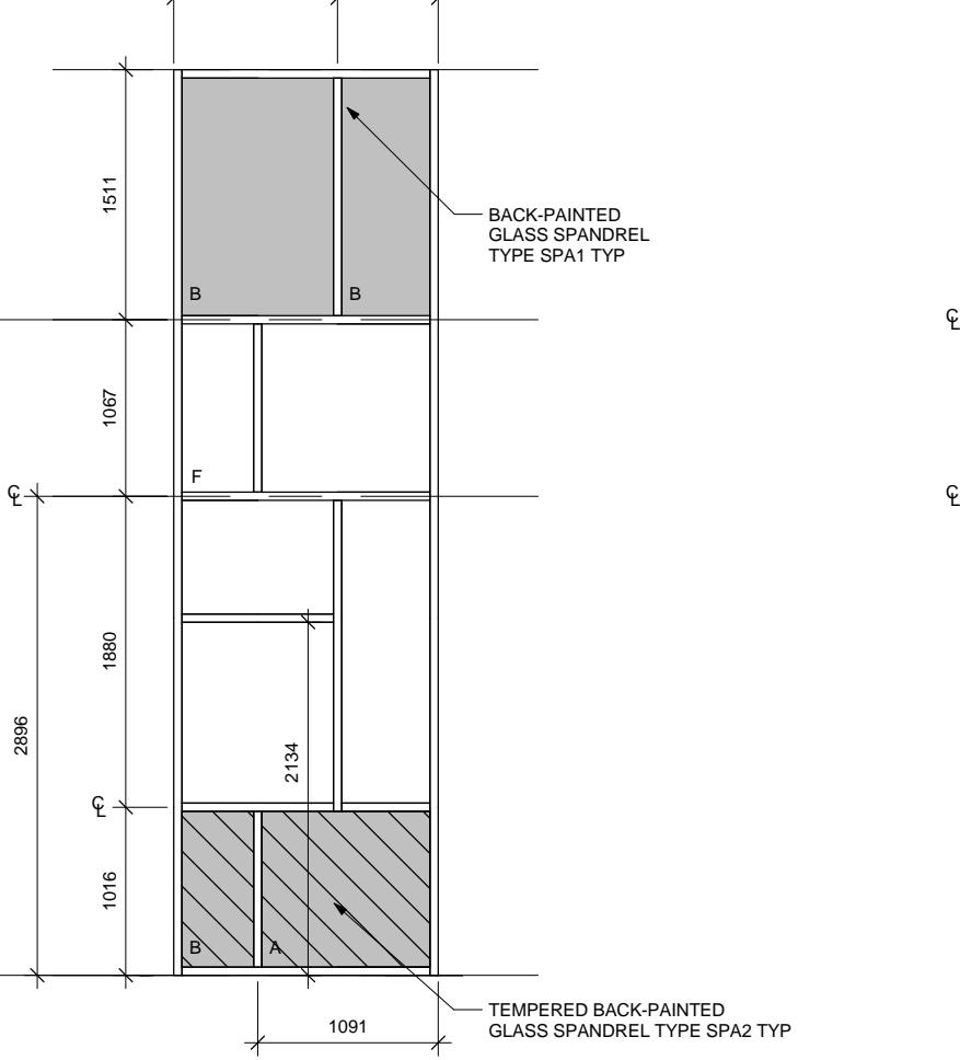
5 CURTAIN PANEL NORTH 3 1:50
