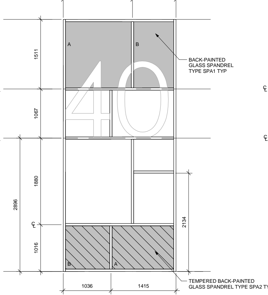
6 CURTAIN PANEL WEST 1:50
