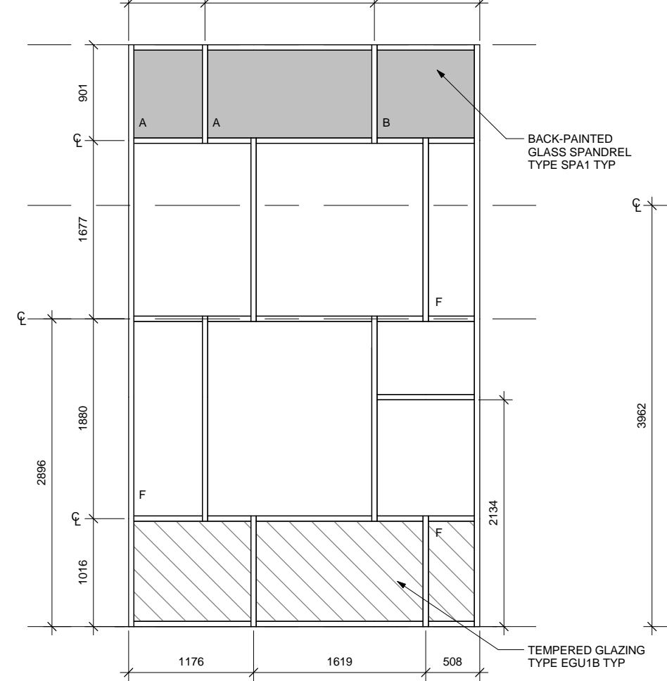
4 CURTAIN PANEL NORTH 2 1:50
