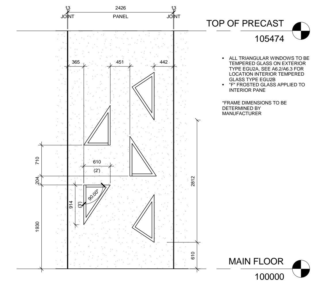
9 PANEL WINDOW LAYOUT / TYPE 1:50
