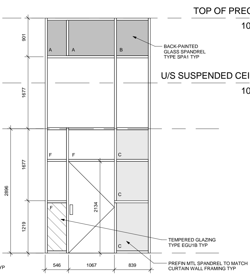
7 CURTAIN PANEL EAST 1:50
