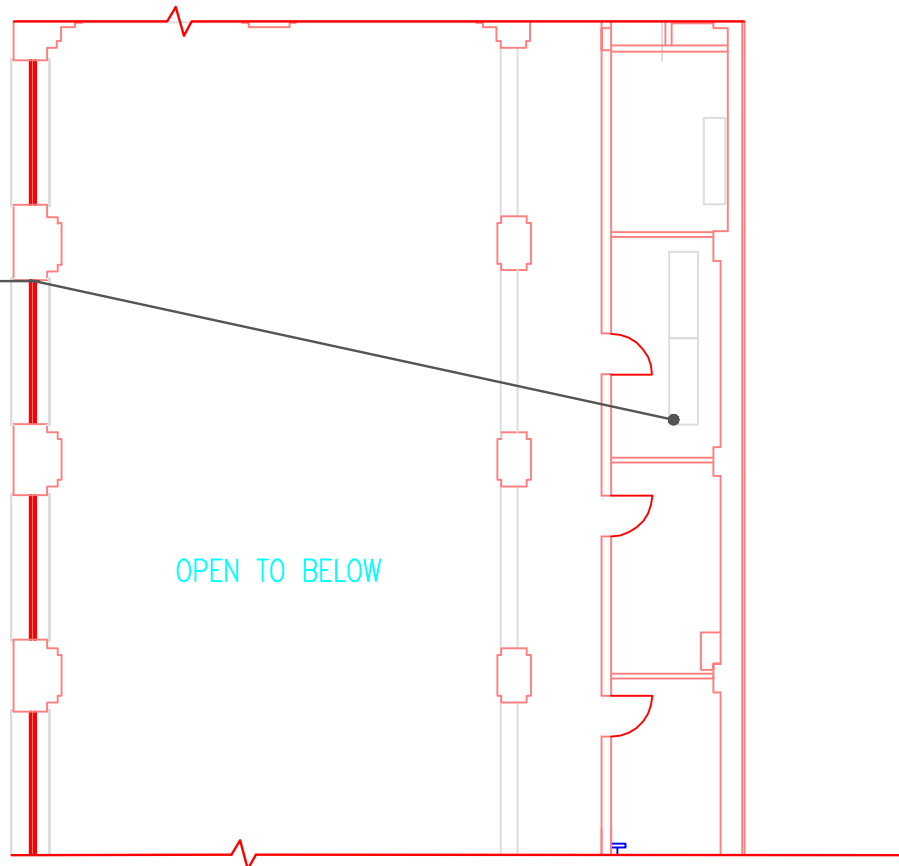
A PARTIAL MEZZANINE FLOOR PLAN
