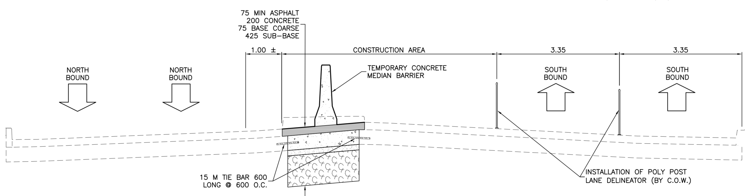
A PHASE 1A SECTION SCALE H = 1 : 50 V = 1:25
