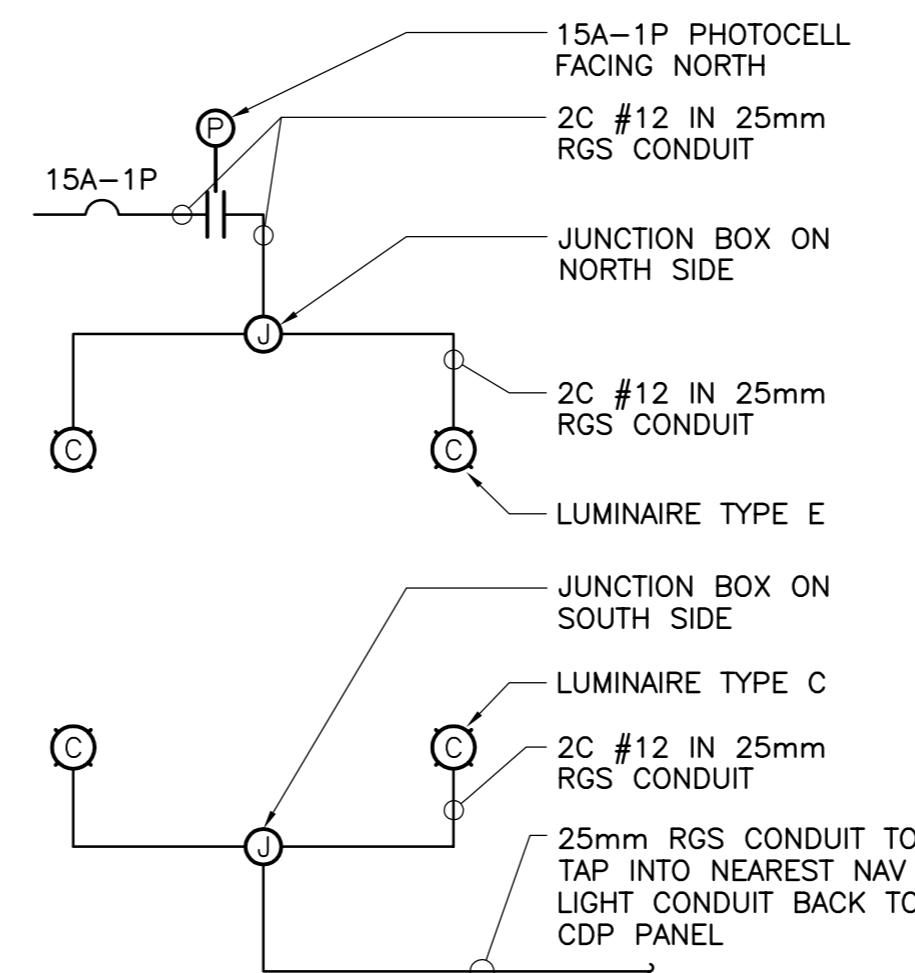
2 UNDERBRIDGE LUMINAIRE WIRING DIAGRAM N.T.S.
