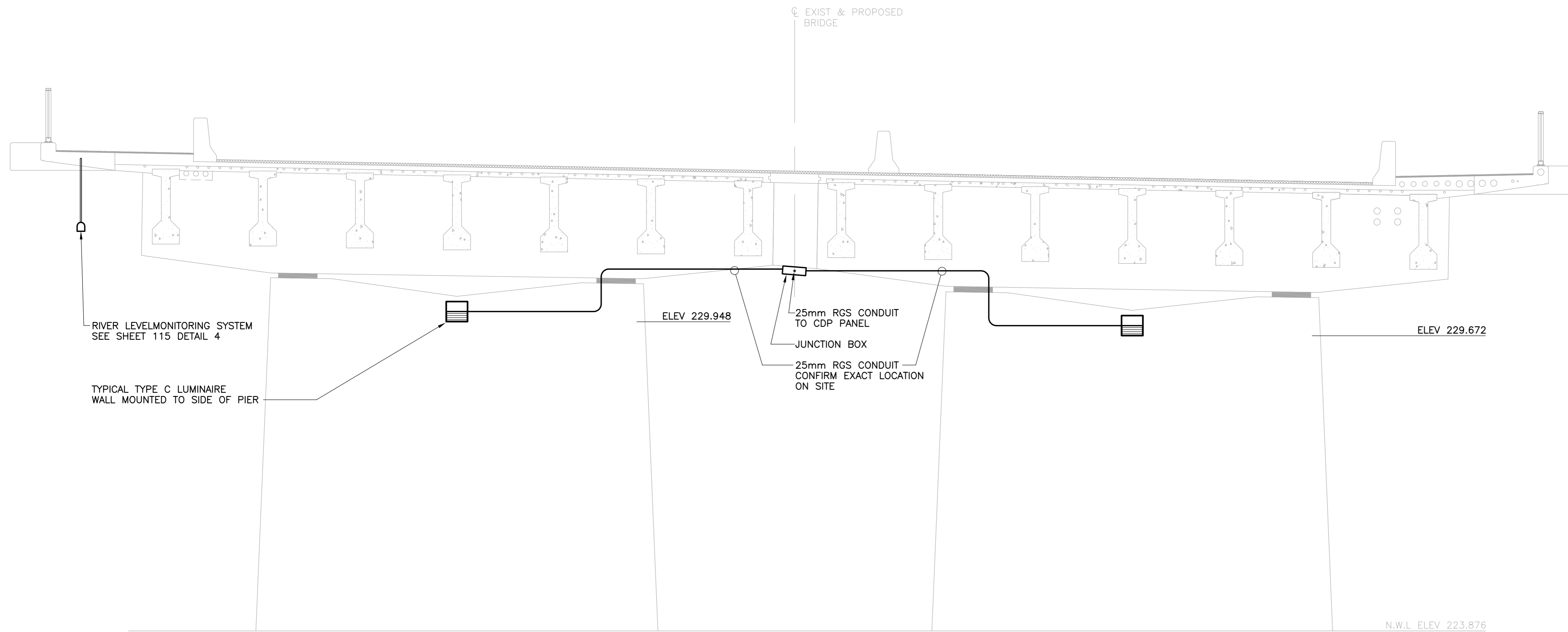
1 UNDERBRIDGE LIGHTING DETAIL - NORTH SIDE 1 : 50 SIMILAR FOR SOUTH SIDE
