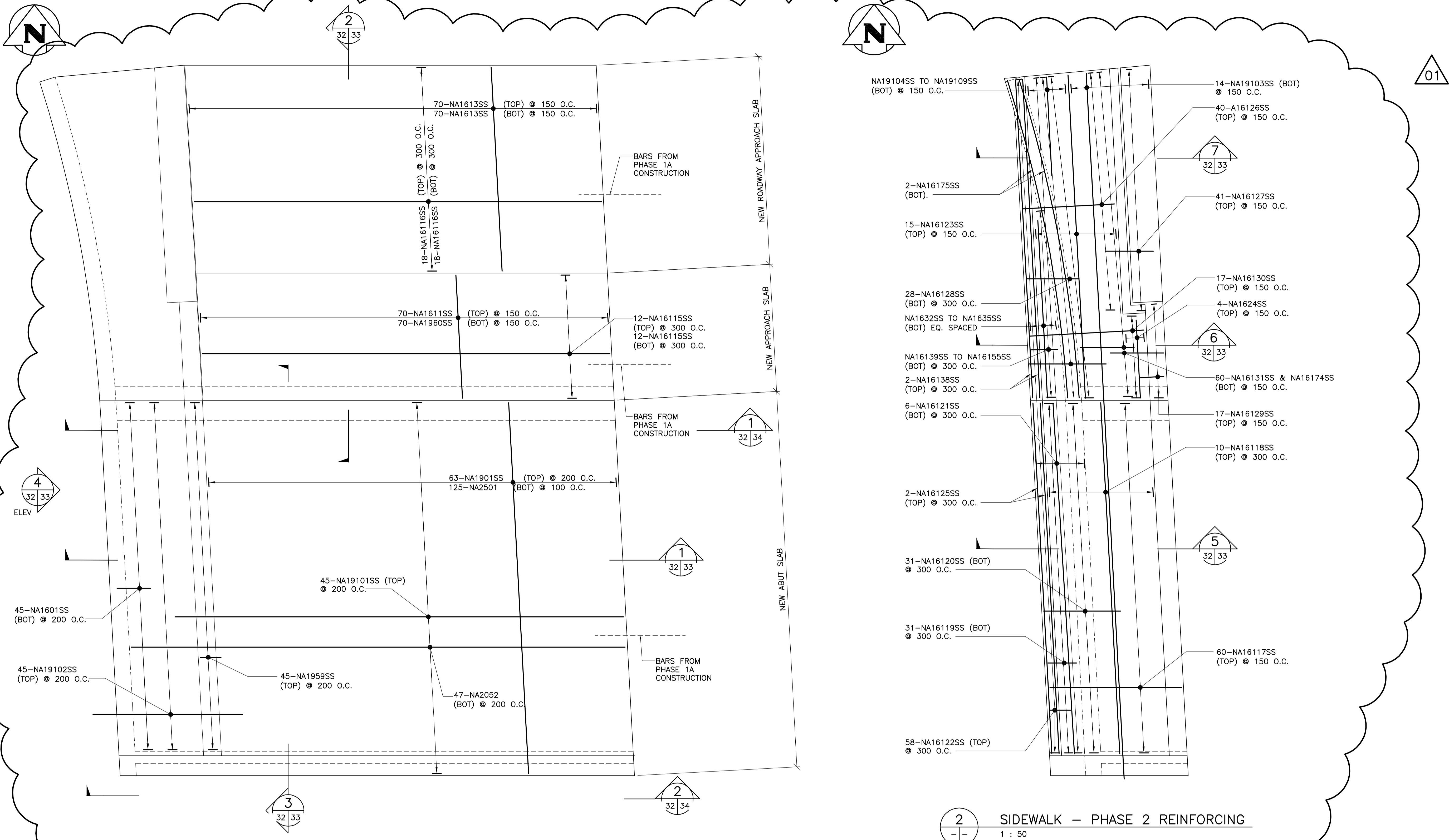
1 ABUTMENT ROOF SLAB - PHASE 2 REINFORCING 1 : 50
