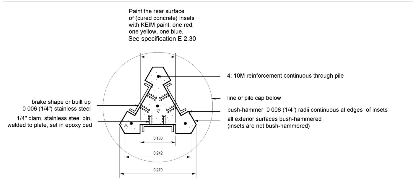
DETAIL 2 - SECTION - BOLLARD
