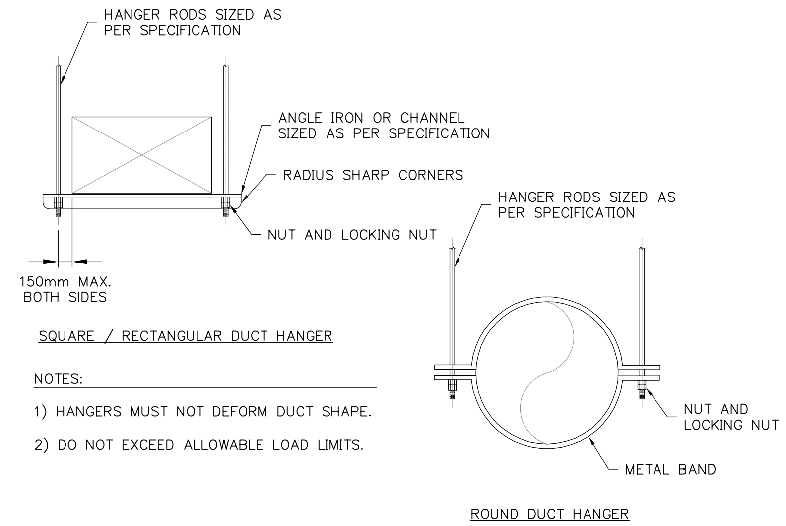
DETAIL 3 SCALE: NTS DUCTWORK SUPPORT AND HANGER DETAIL
