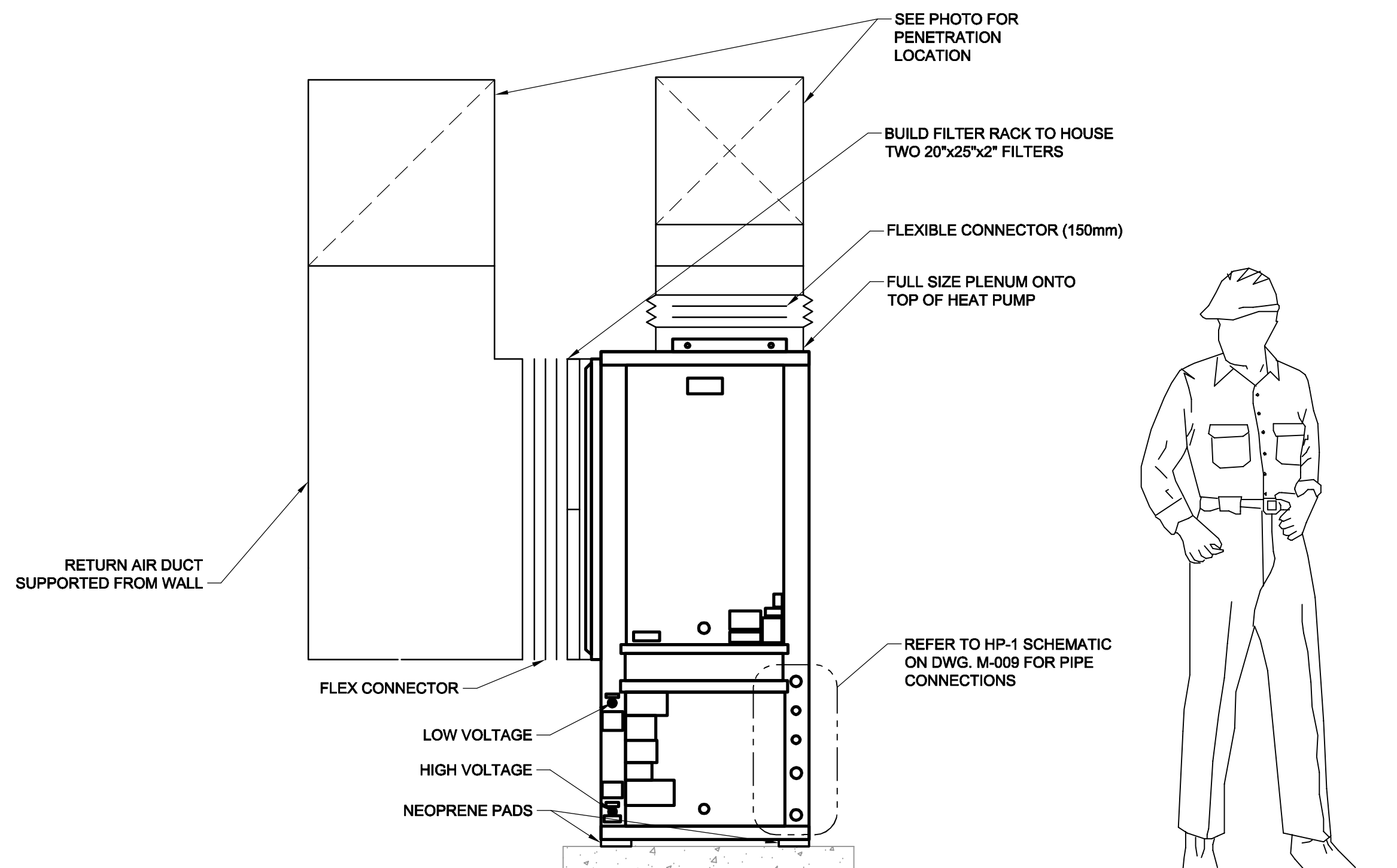
DETAIL 5 SCALE: NTS HP-1 VENTILATION
