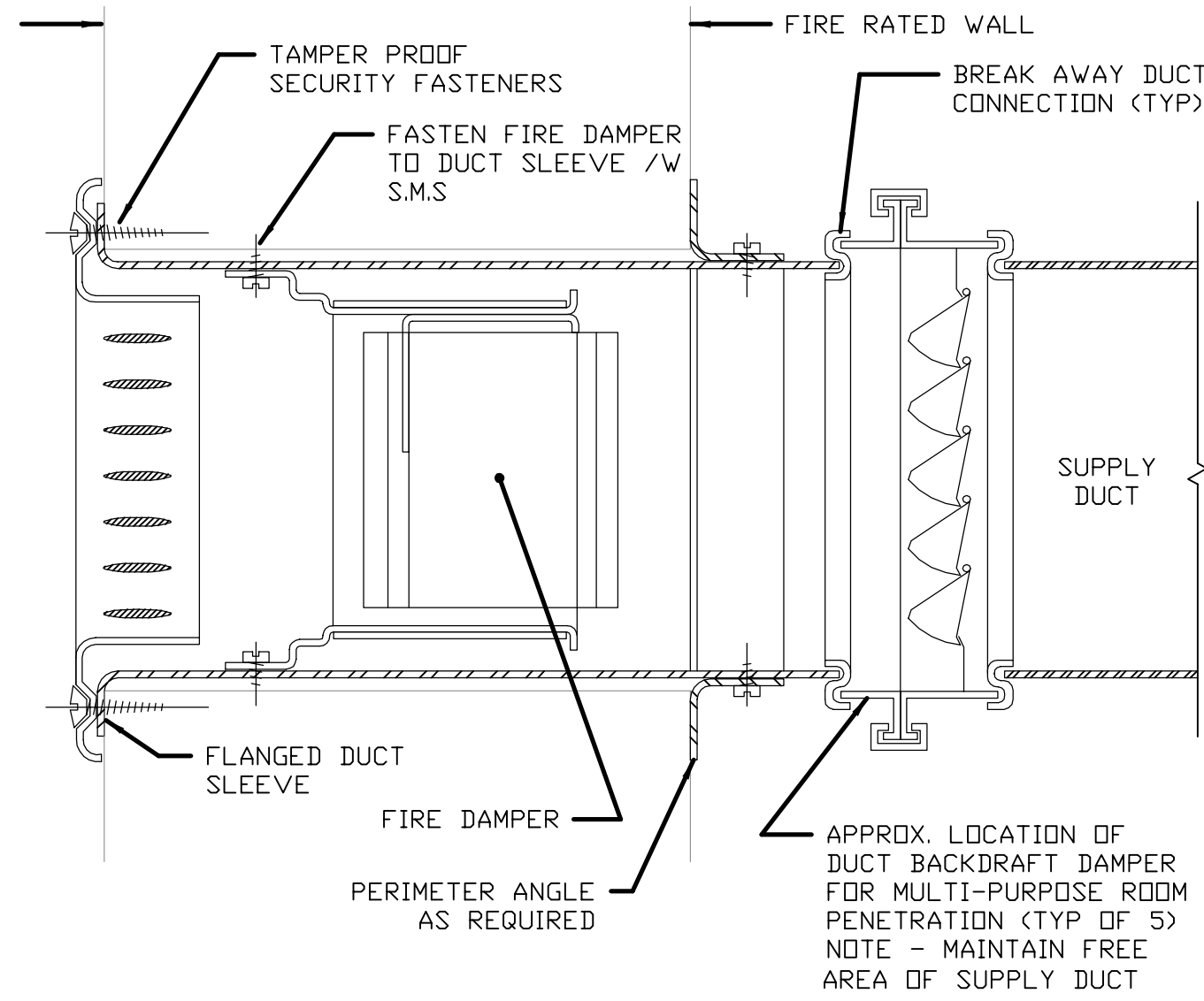
DETAIL 2 SCALE: NTS DIFFUSER OR GRILLE FIREWALL PENETRATION
