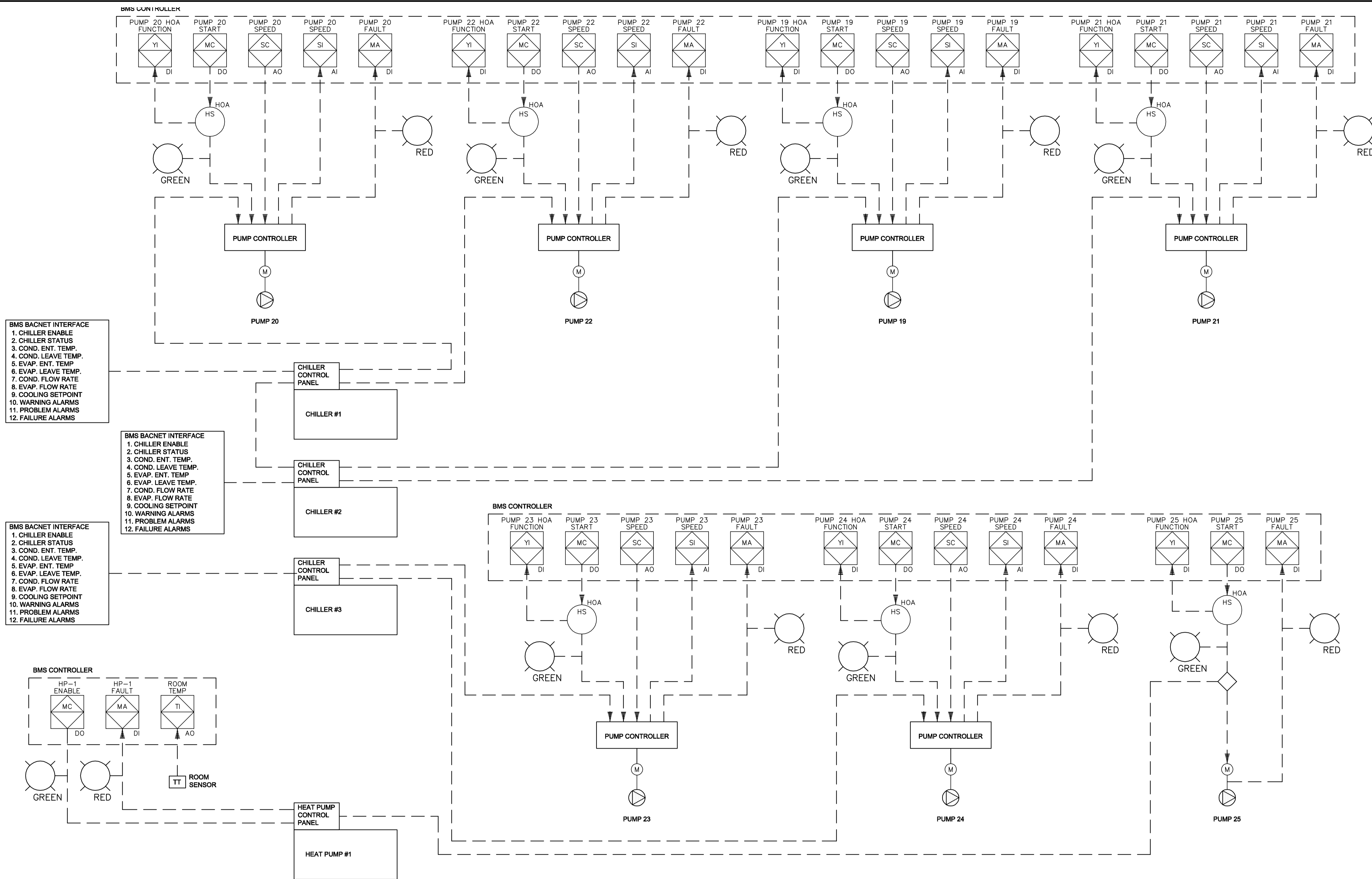
SCHMATIC 1 SCALE: NTS CHILLER PUMP SCHEMATIC
