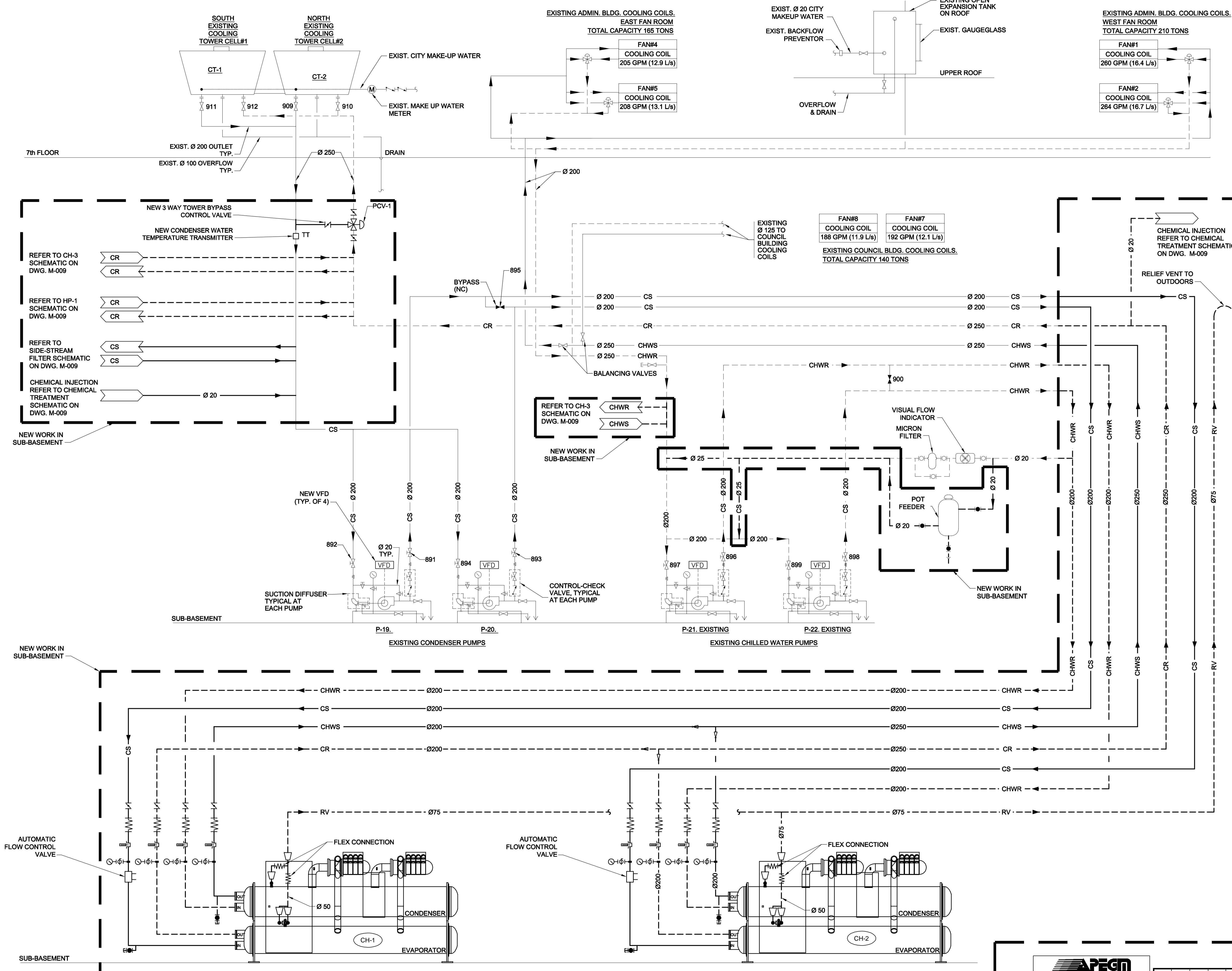
CHILLER HYDRONIC SCHEMATIC SCALE: NTS
