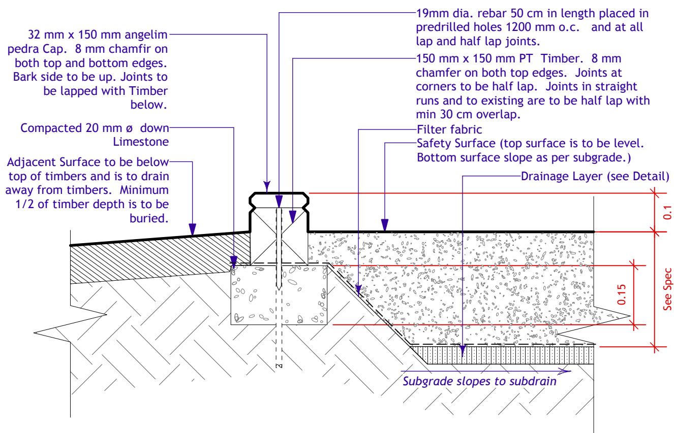
3 Timber Play Curb (Single Layer w. Cap) L-7 Scale: 1:10
