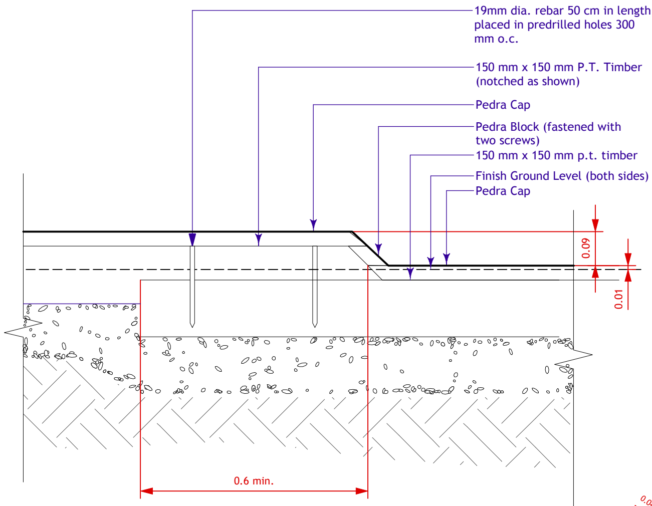
1 Timber Play Curb (accessible entry point) L-7 Scale: 1:10
