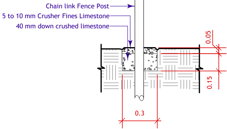
2 Chain Link Fence Post in Gravel Paving L-10 Scale: 1:20
