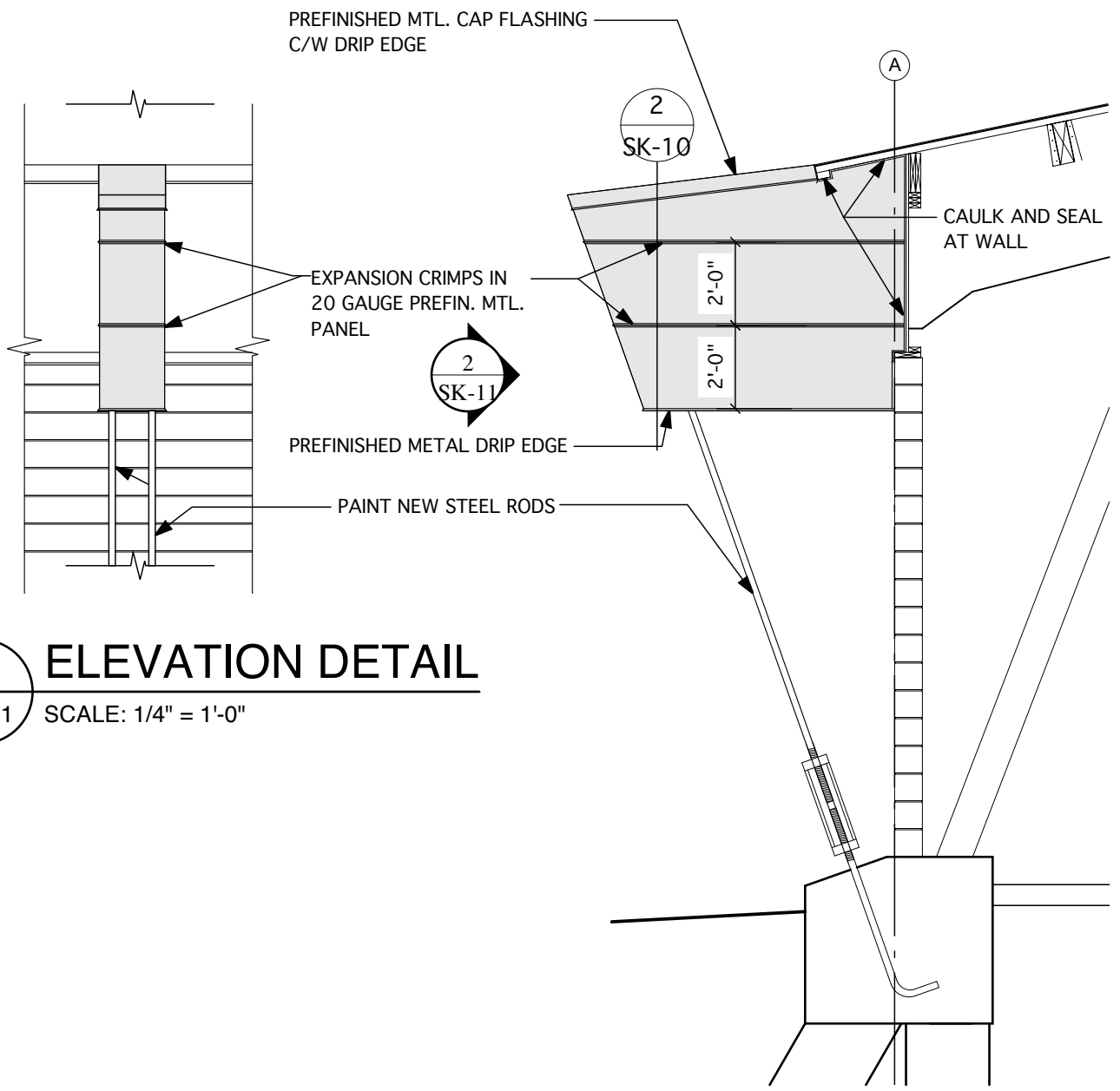
1 ELEVATION DETAIL SK-11 SCALE: 1/4" = 1'-0"
