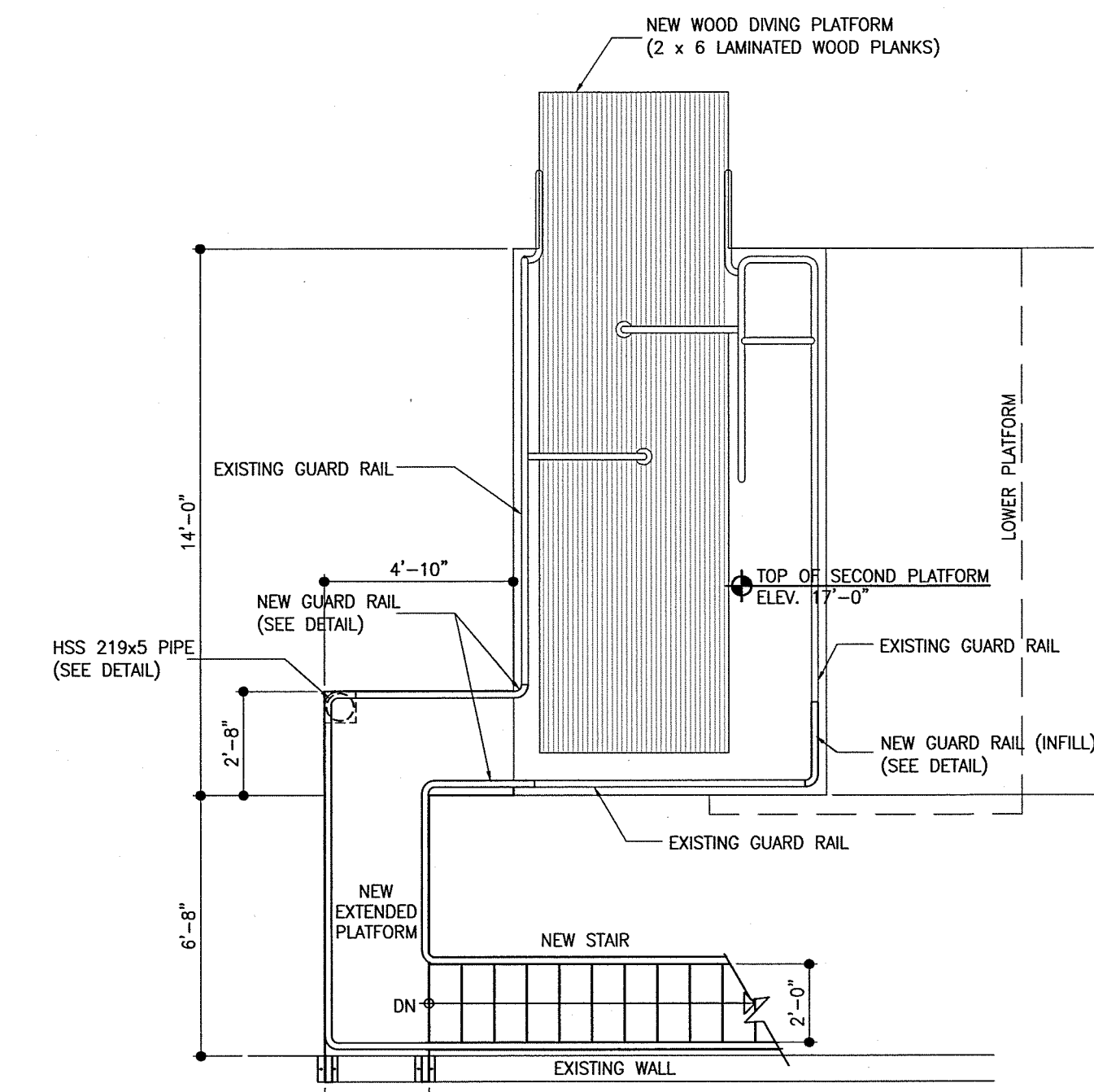
F NEW STAIR PLAN AT SECOND PLATFORM LEVEL S01 1/4" = 1'-0"
