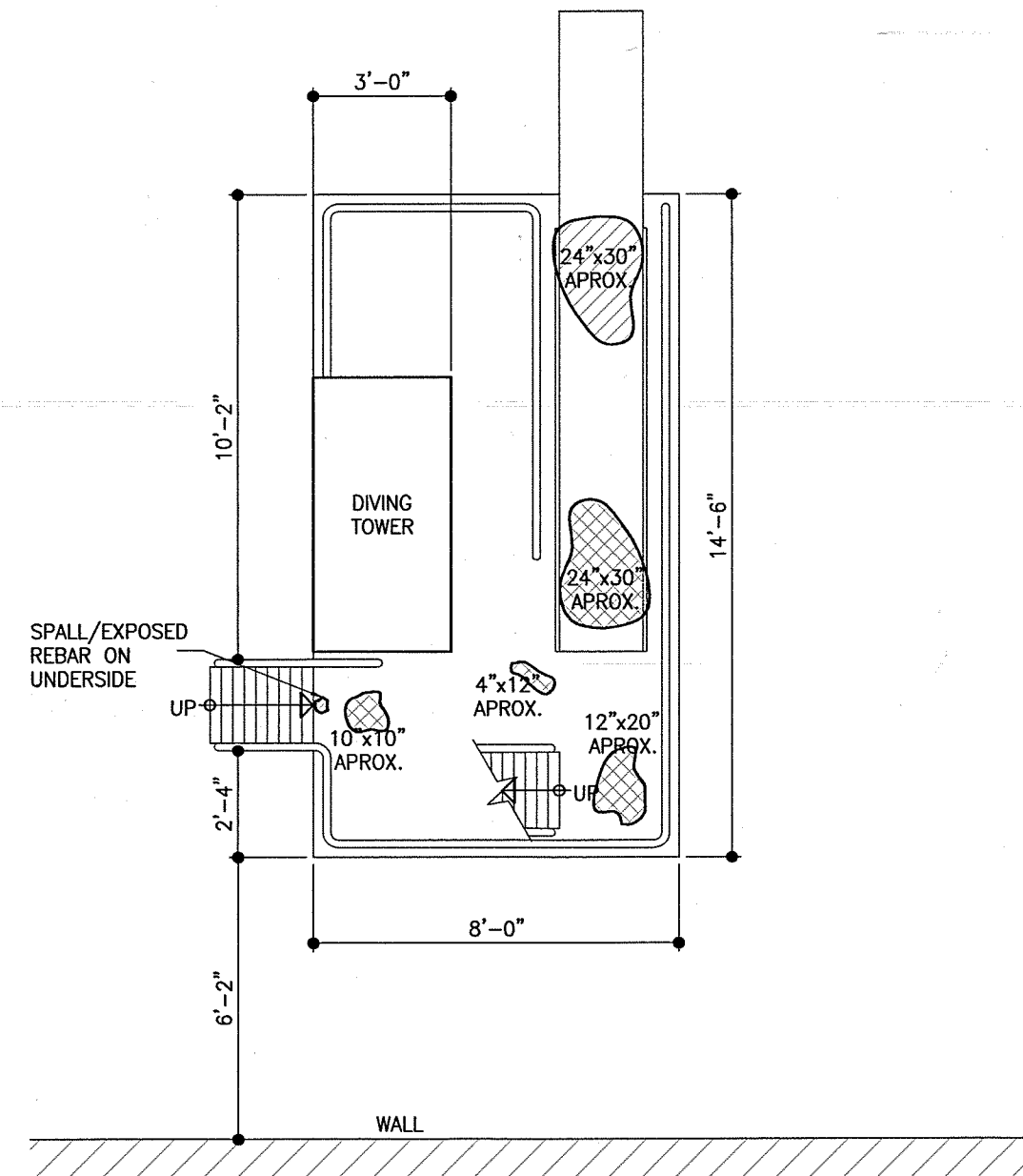
B EXISTING PLAN AT FIRST PLATFORM LEVEL S01 1/4" = 1'-0"
