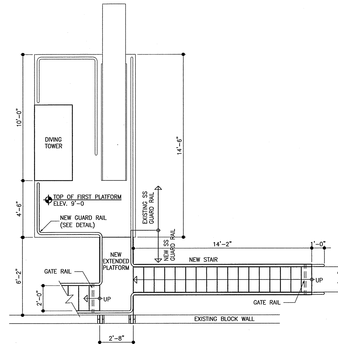
E NEW STAIR PLAN AT FIRST PLATFORM LEVEL S01 1/4" = 1'-0"
