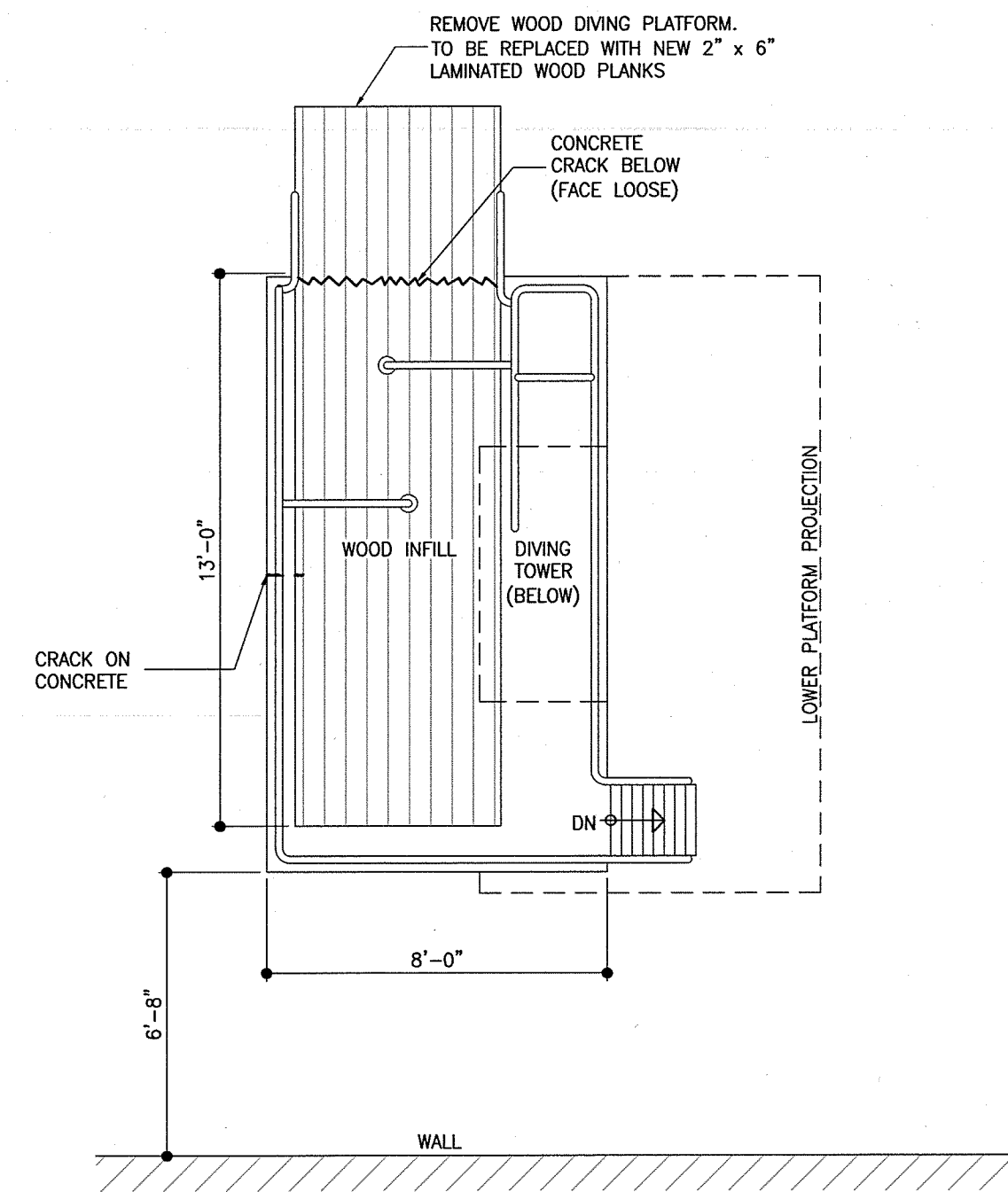
C EXISTING PLAN AT SECOND PLATFORM LEVEL S01 1/4" = 1'-0"
