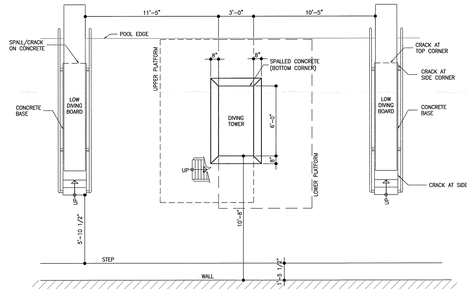
A EXISTING PLAN AT GROUND LEVEL S01 1/4" = 1'-0"
