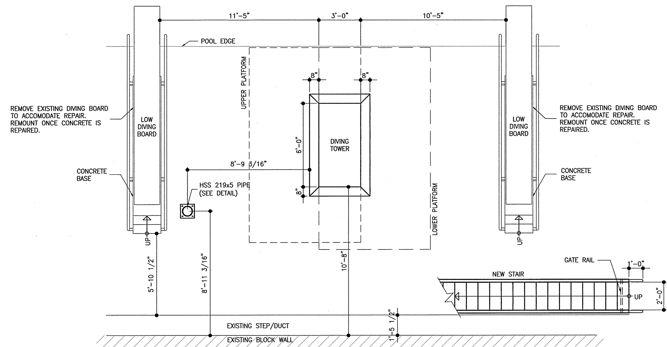
D NEW STAIR PLAN AT GROUND LEVEL S01 1/4" = 1'-0"
