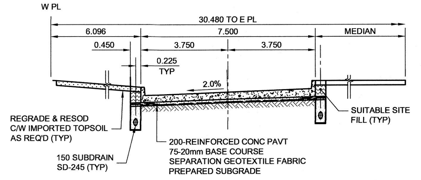
PAVT SECTION CONCRETE PAVEMENT STRUCTURE TYPICAL SCALE: N.T.S.
