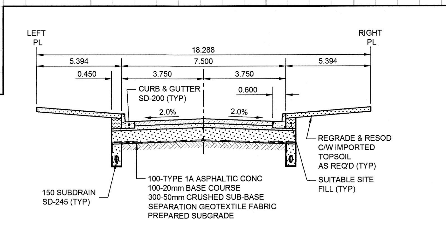
PAVT SECTION ASPHALT PAVEMENT STRUCTURE TYPICAL SCALE: N.T.S
