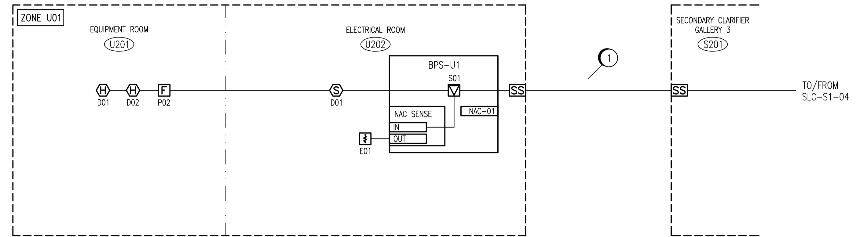
DETECTION RISER DIAGRAM SCALE: NTS
