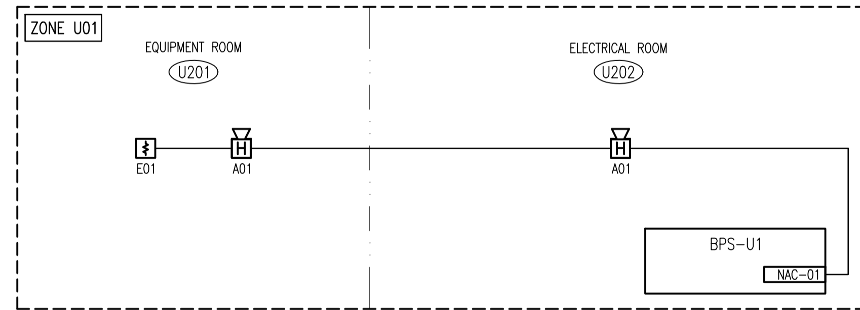
NOTIFICATION RISER DIAGRAM SCALE: NTS
