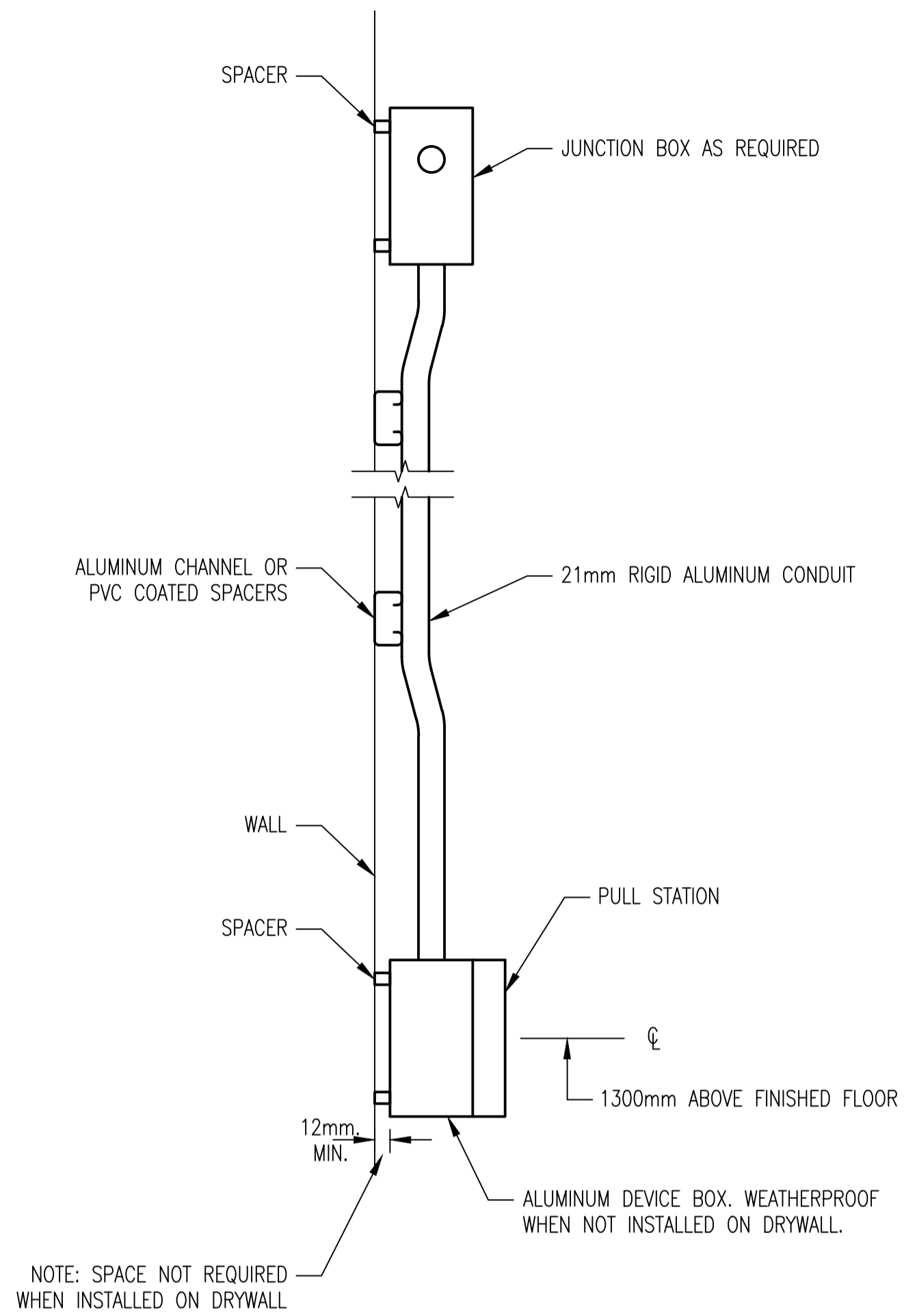
1 PULL STATION DETAIL - CLASS 1, ZONE 2 SCALE 1:4
