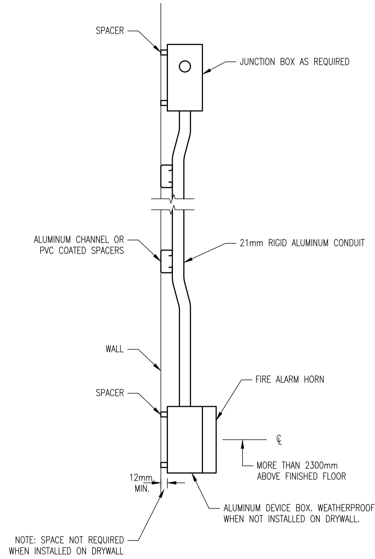
2 AUDIBLE SIGNAL DEVICE - UNCLASSIFIED LOCATION SCALE 1:4
