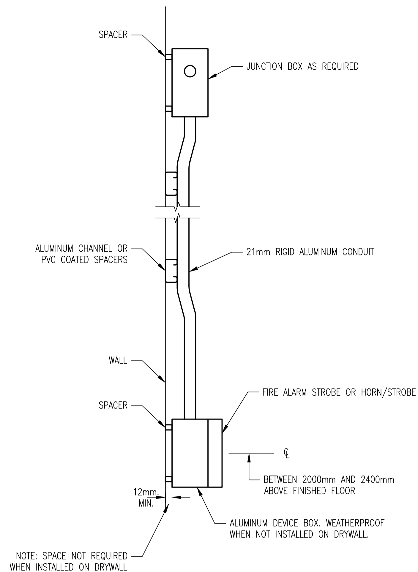
3 VISIBLE SIGNAL DEVICE - UNCLASSIFIED LOCATION SCALE 1:4
