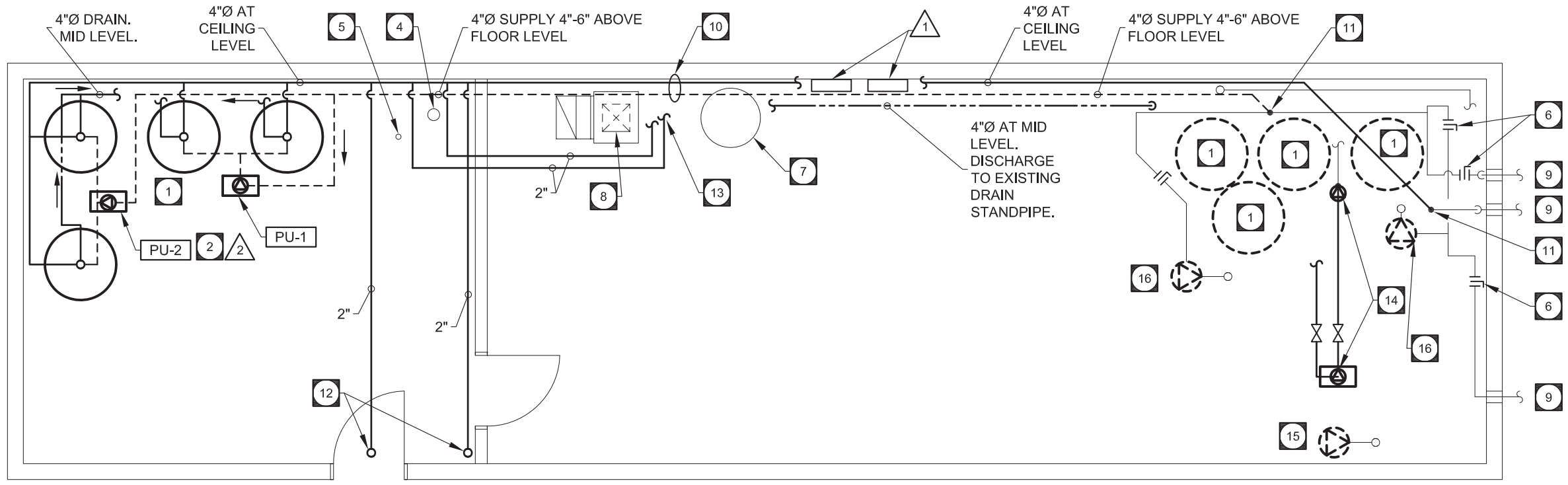
1 MECHANICAL ROOM PLAN M-1 SCALE: 3/16" = 1' - 0"
