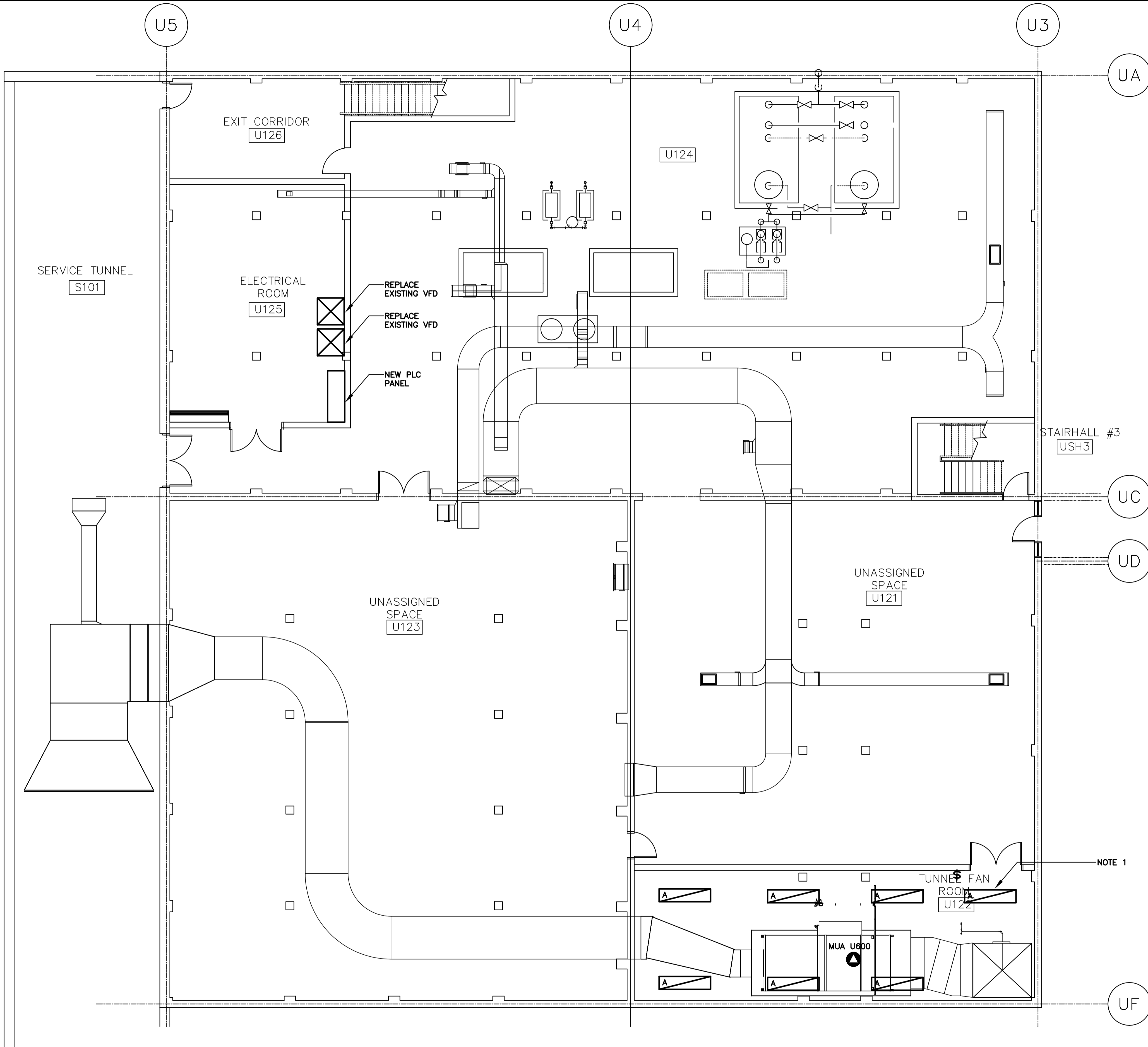
1 AREA U - UTILITY LOWER LEVEL PLAN SCALE 1:75
