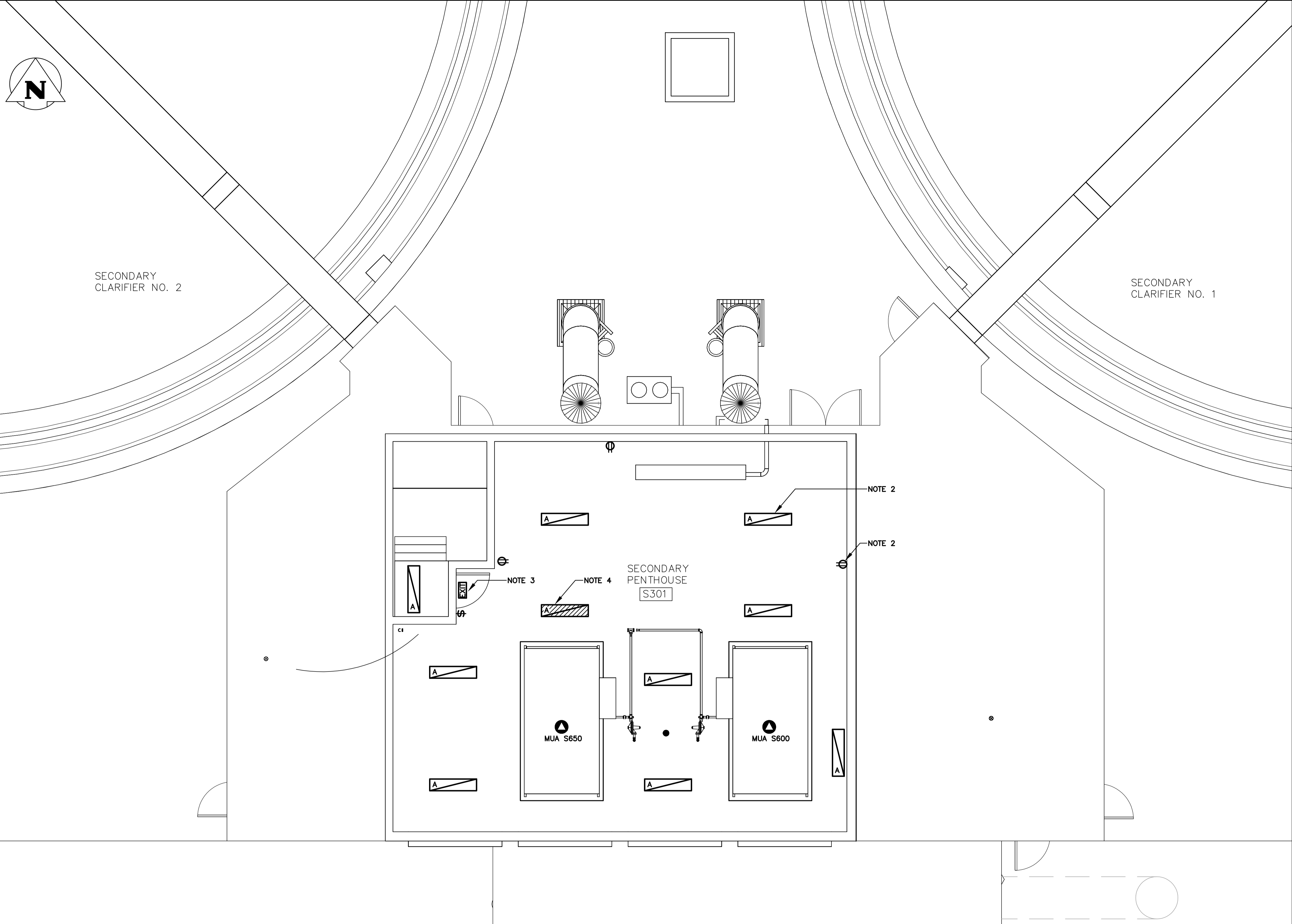
1 AREA S - PENTHOUSE PLAN SCALE 1:50
