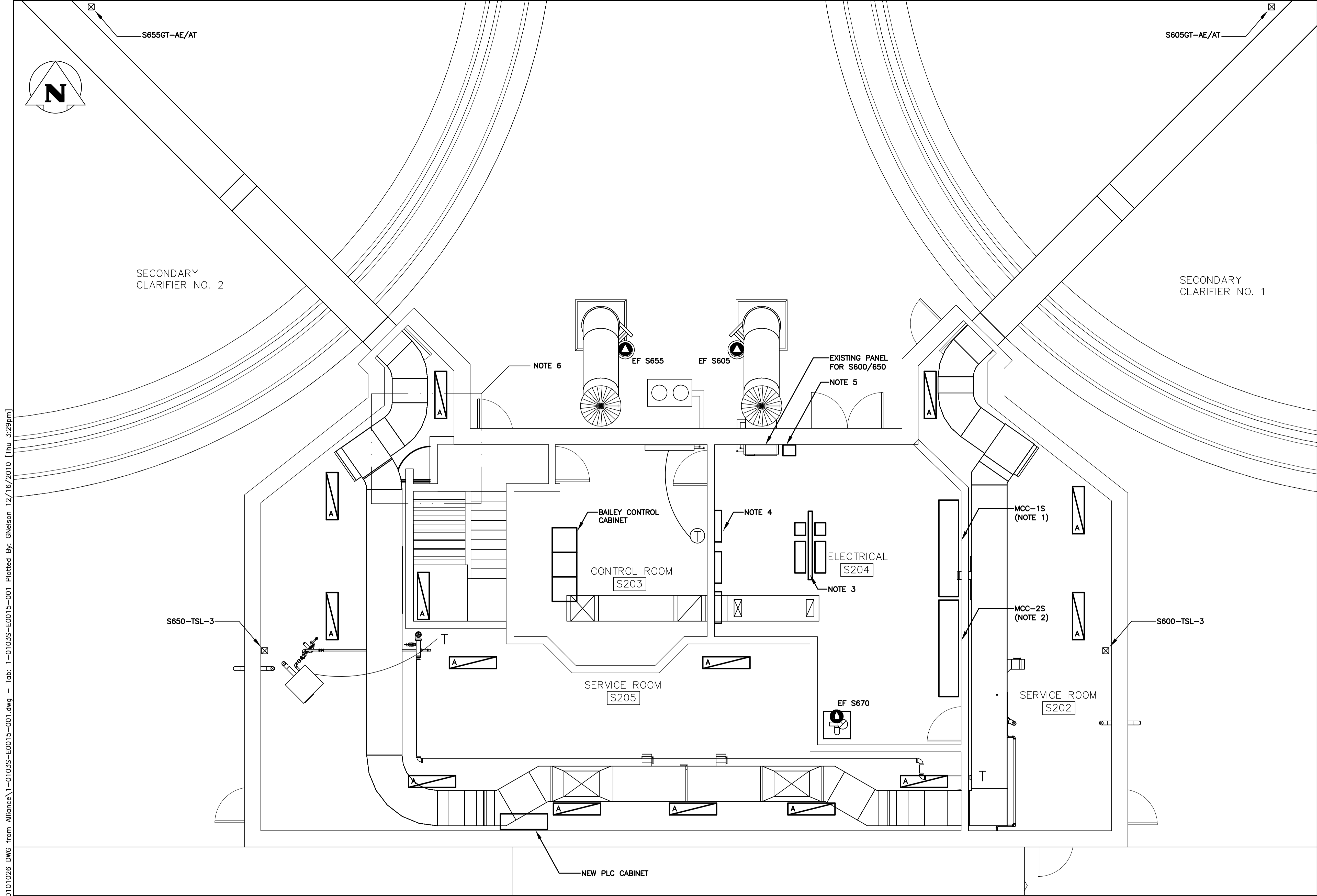
1 AREA S - DISTRIBUTION BUILDING PLAN SCALE 1:50
