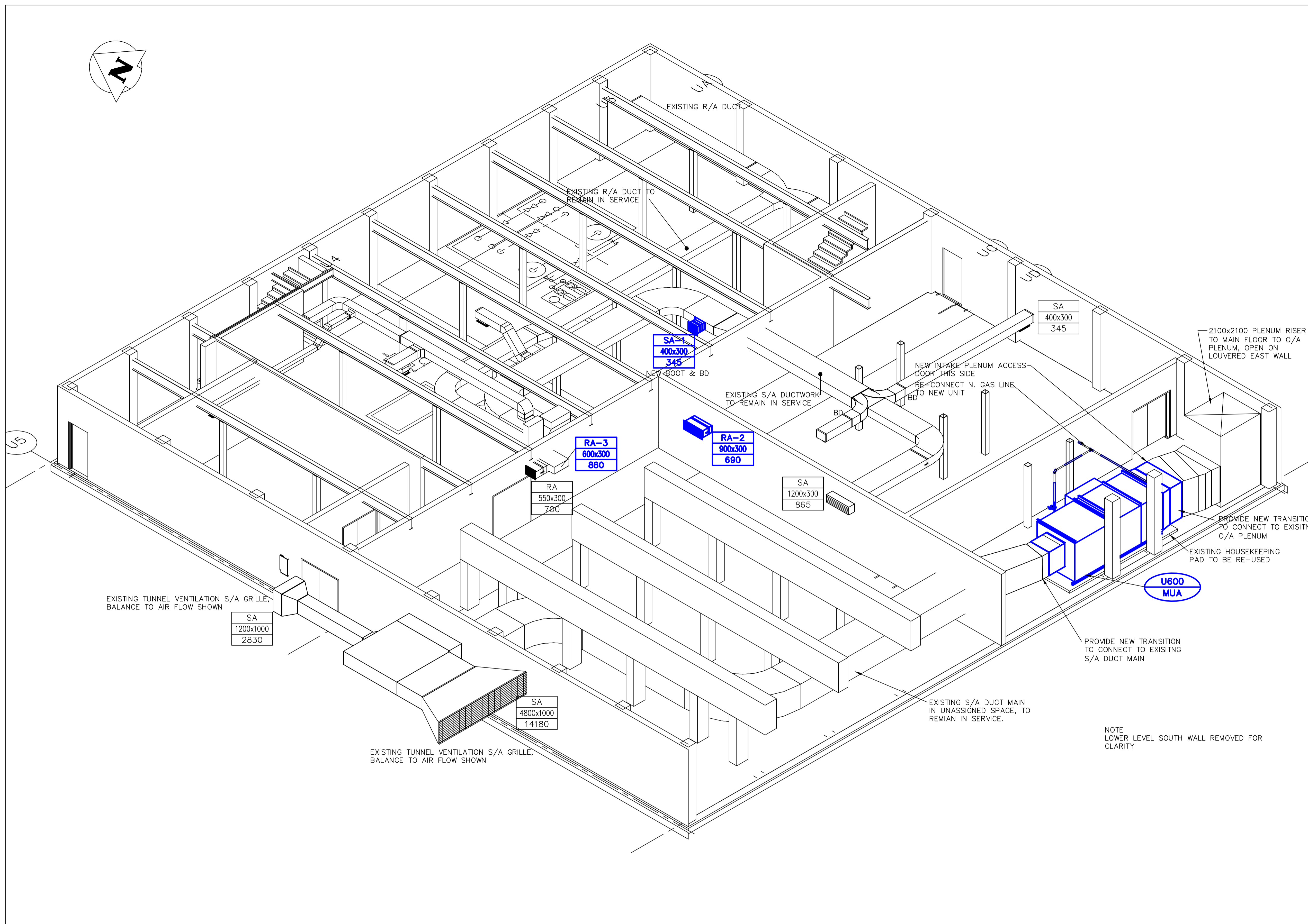
A AREA U – UTILITY LOWER LEVEL VENTILATION – NEW CONDITIONS ISOMETRIC - NTS
