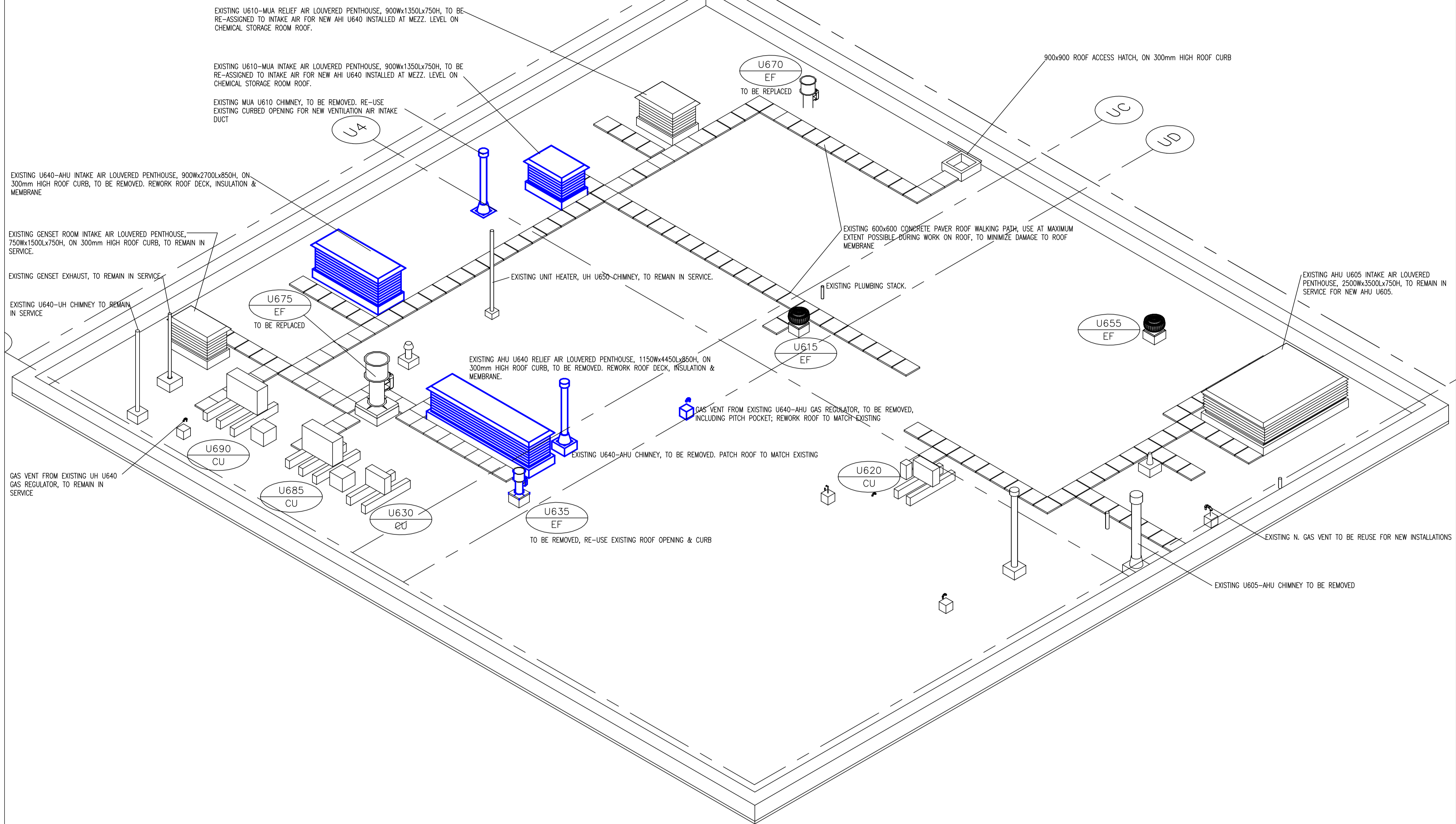
(A) AREA U UTILITY BUILDING ROOF – EXISTING CONDITIONS – ISOMETRIC NTS
