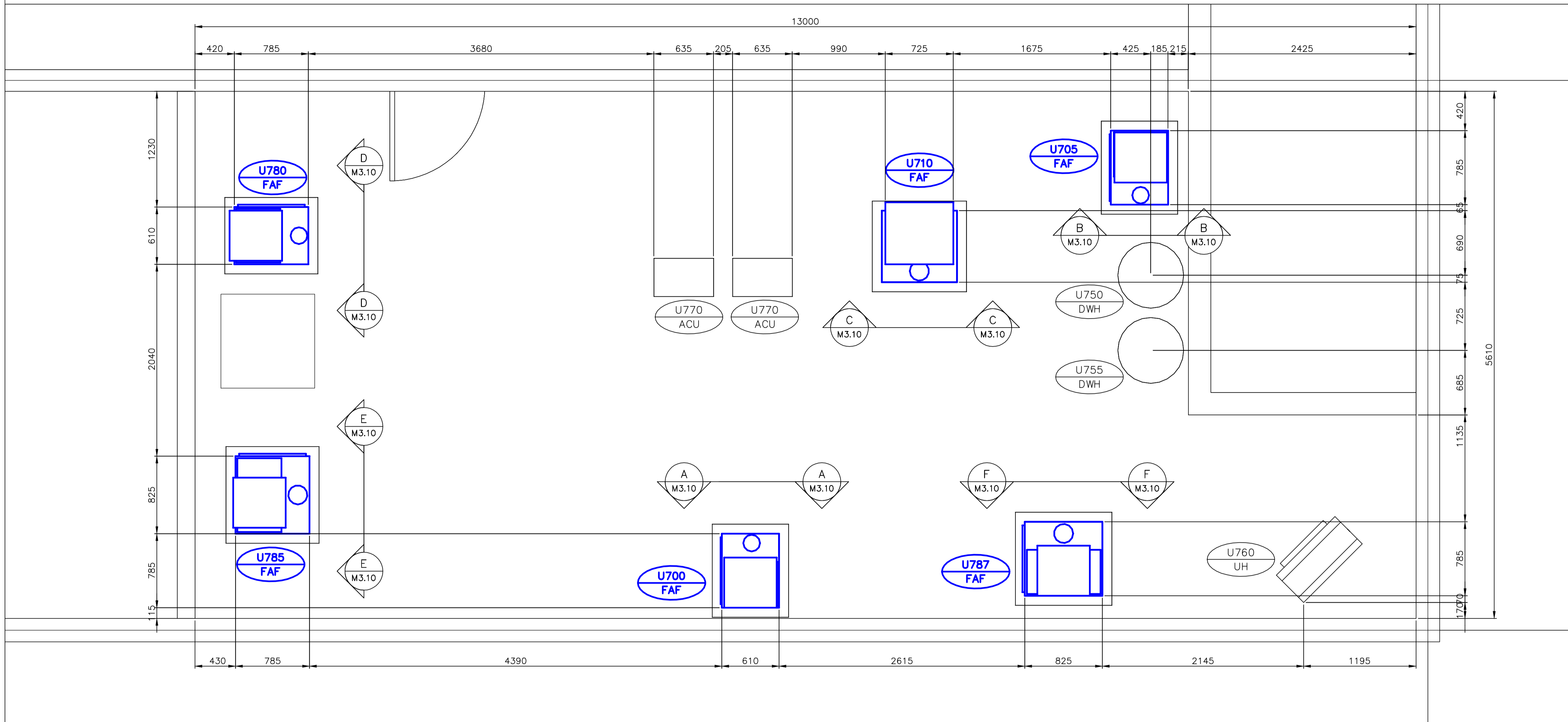
A MECHANICAL ROOM - EQUIPMENT LAYOUT SCALE 1:25
