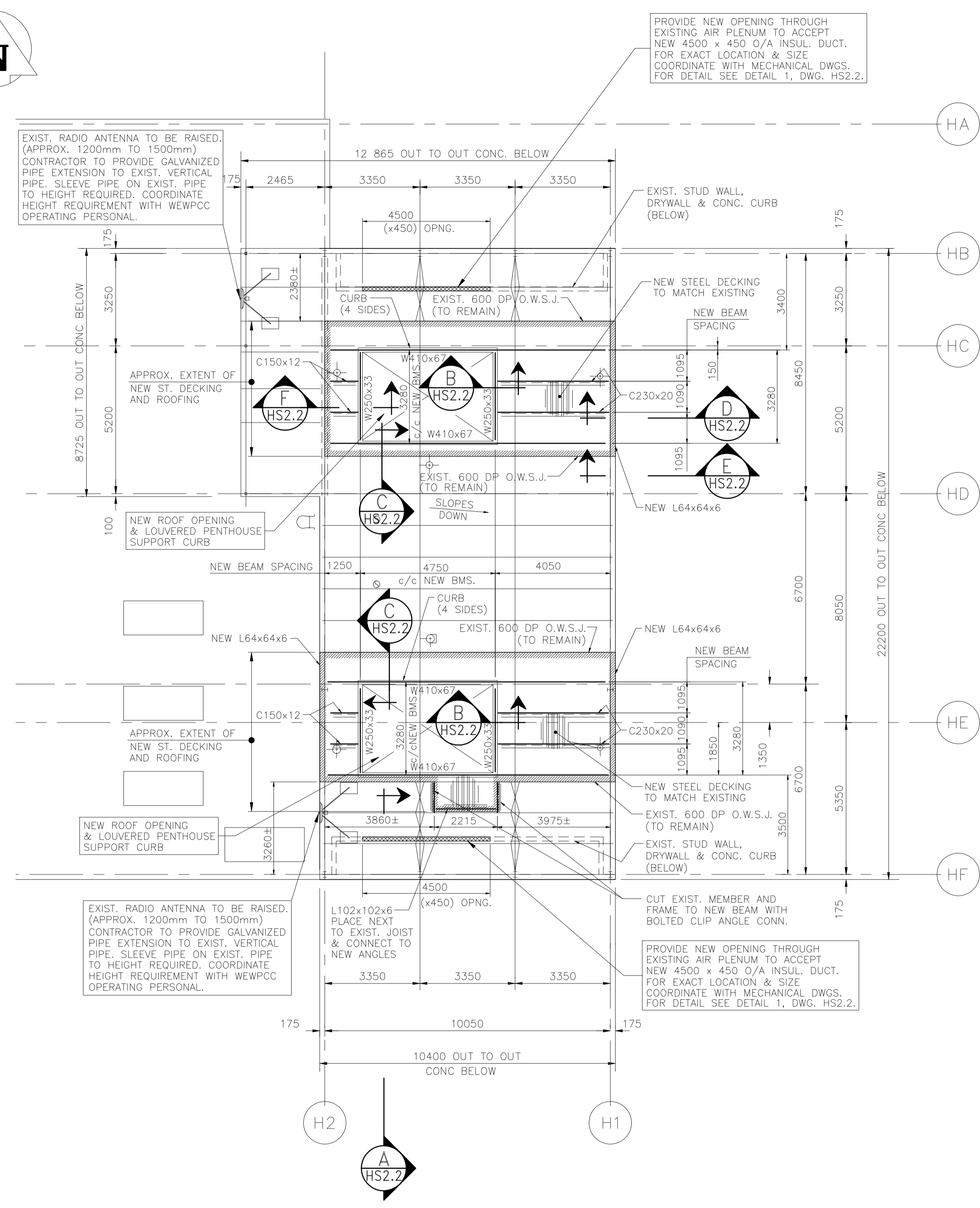
MODIFIED MECHANICAL ROOF PLAN (EL. 252.100)
