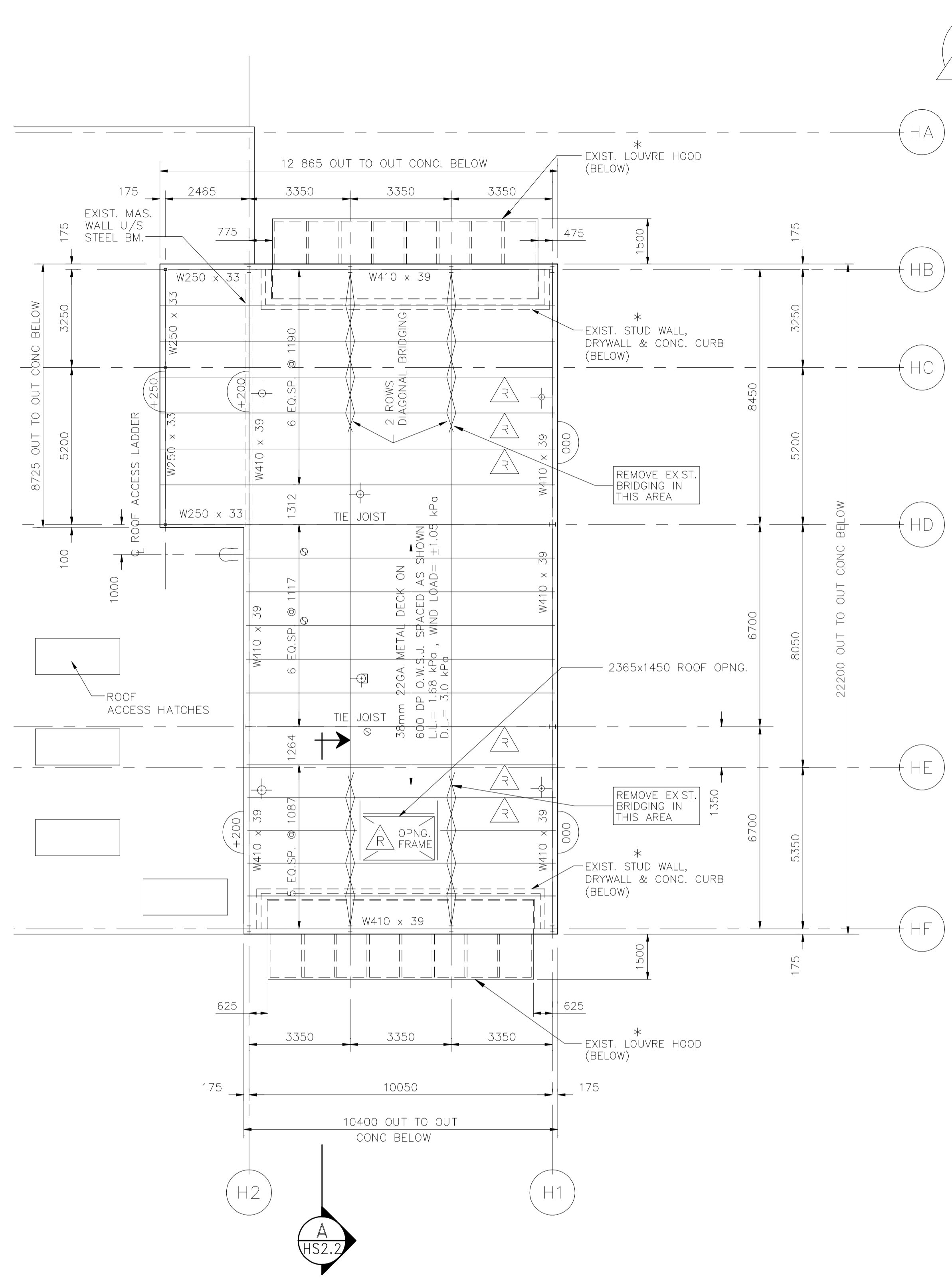
EXISTING MECHANICAL ROOF PLAN (EL. 252.100)
