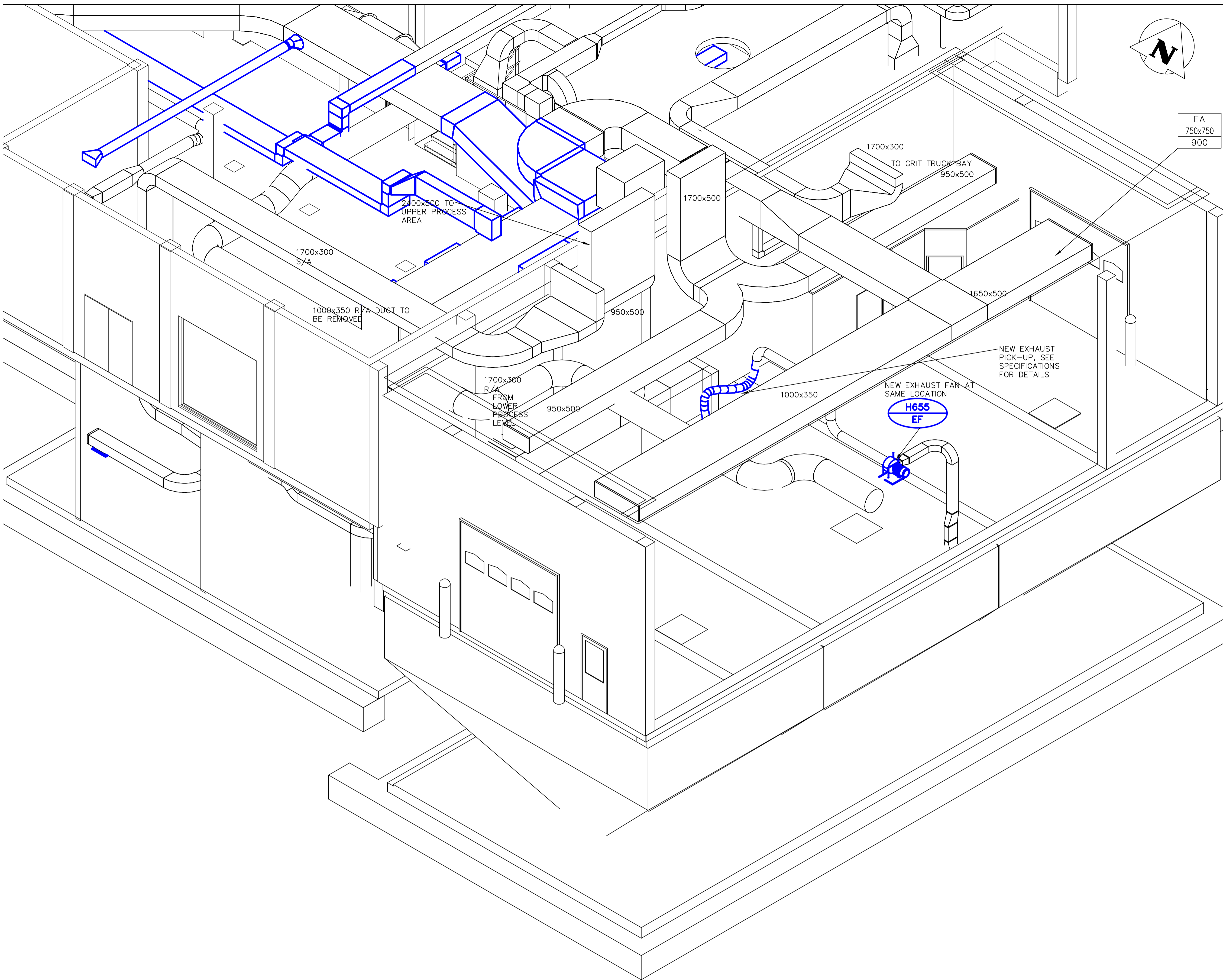
A AREA H - SLUDGE TRUCK BAY MODIFICATIONS - ISOMETRIC - N.T.S.
