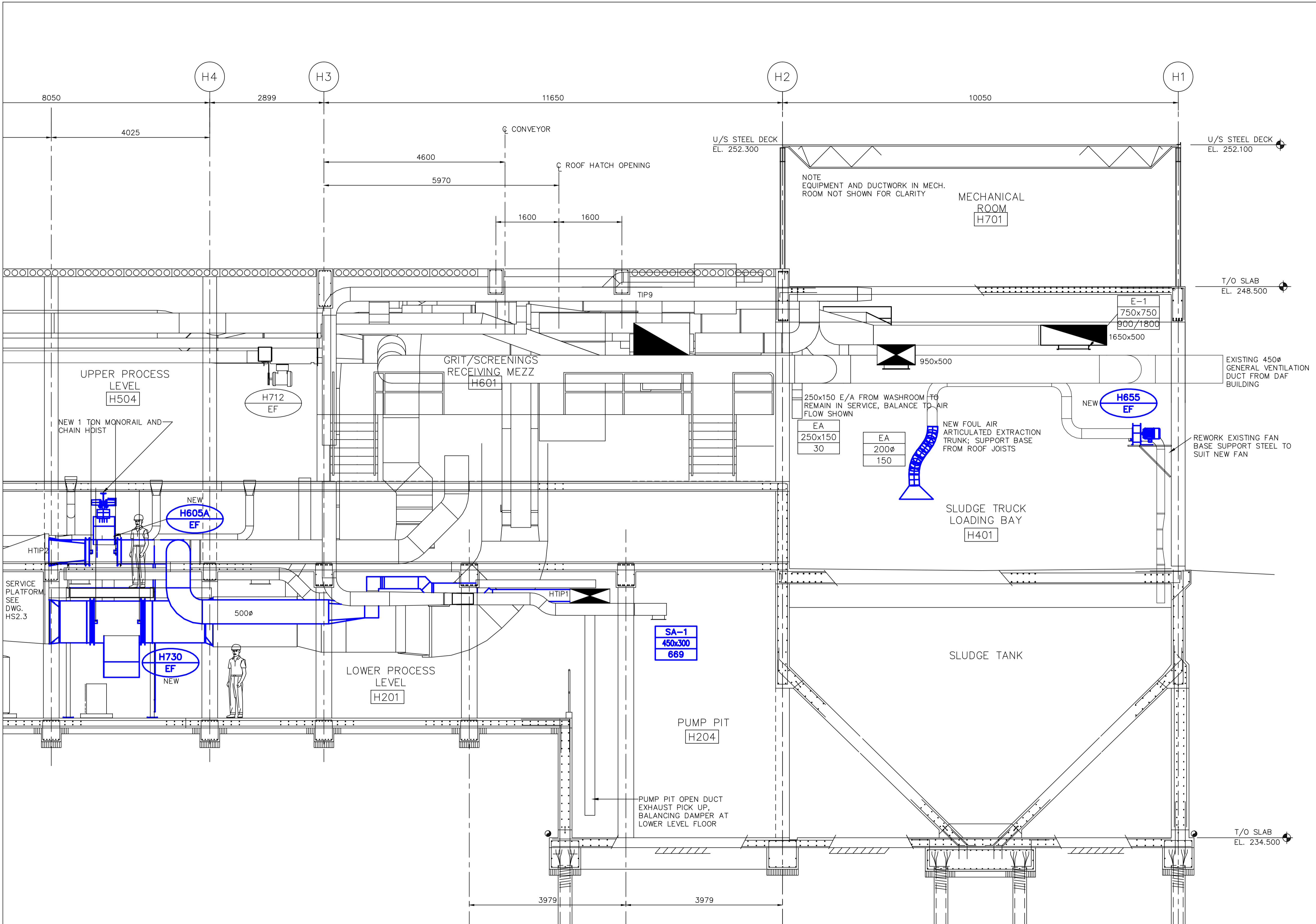
A - AREA H NEW CONDITIONS - SECTION AT GRID LINE HE SCALE 1:50
