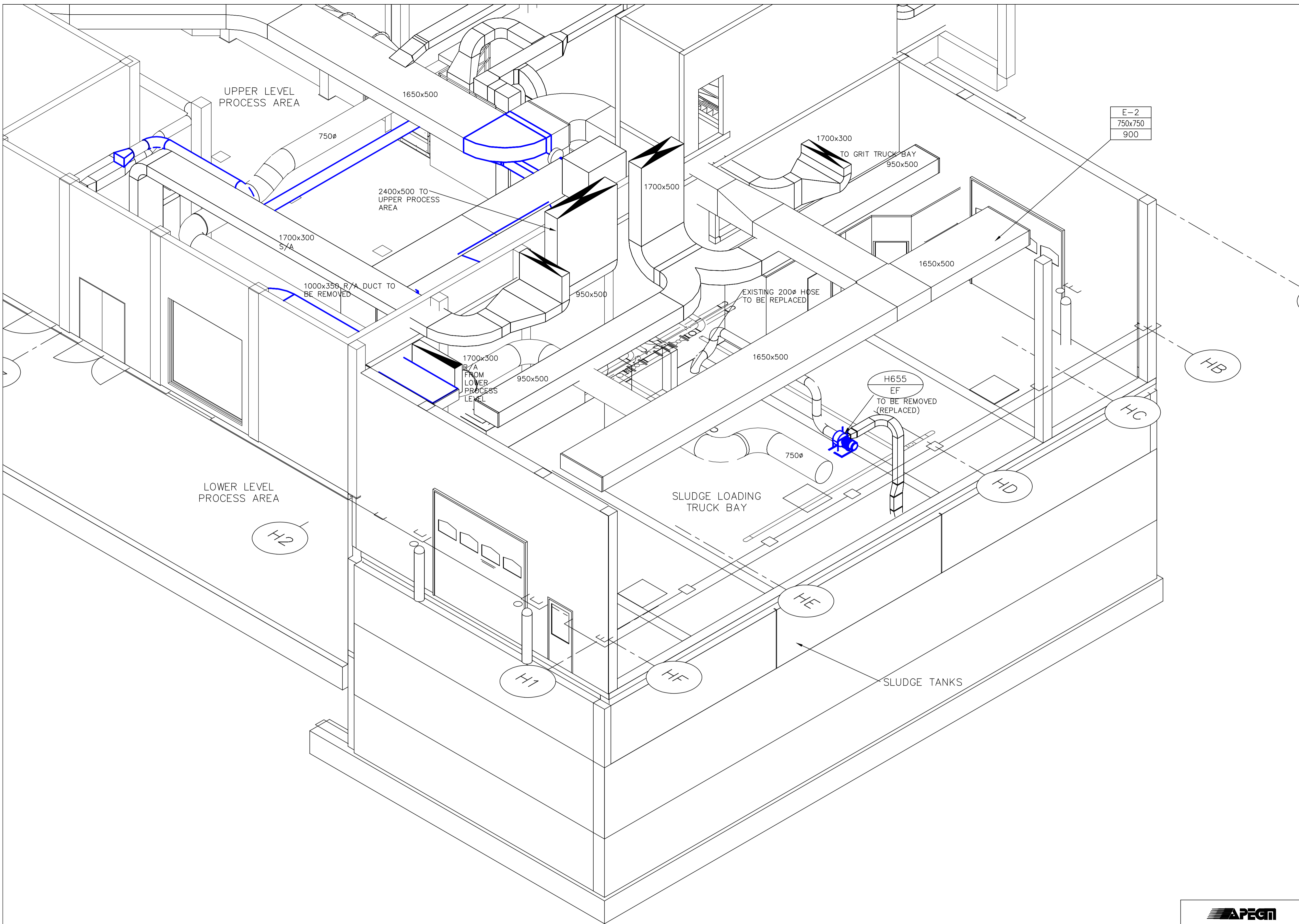
(A) AREA H - SLUDGE LOADING TRUCK BAY VENTILATION - EXISTING CONDITIONS ISOMETRIC - N.T.S.
