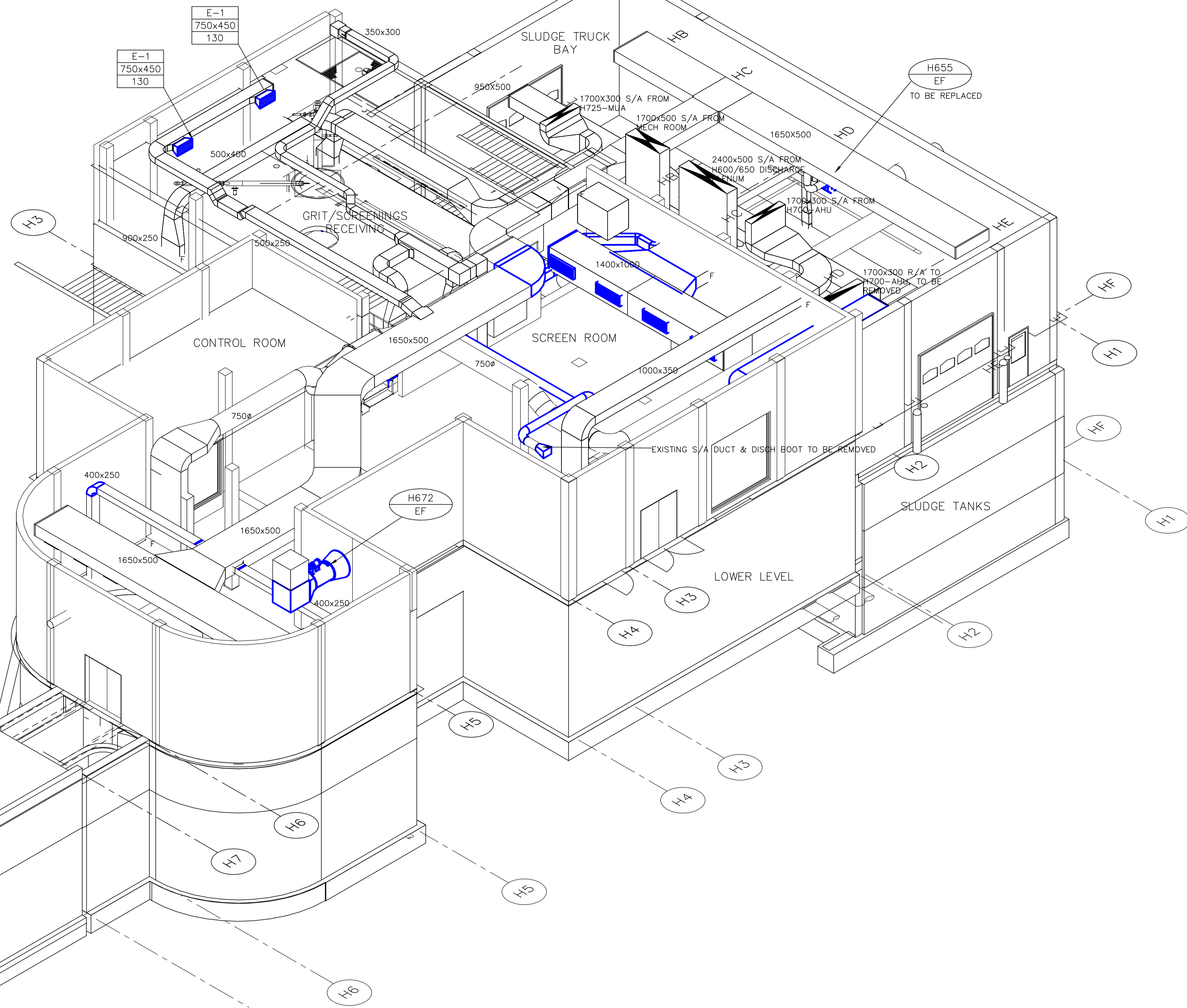
A AREA H - UPPER PROCESS LEVEL VENTILATION - EXISTING CONDITIONS ISOMETRIC N.T.S.
