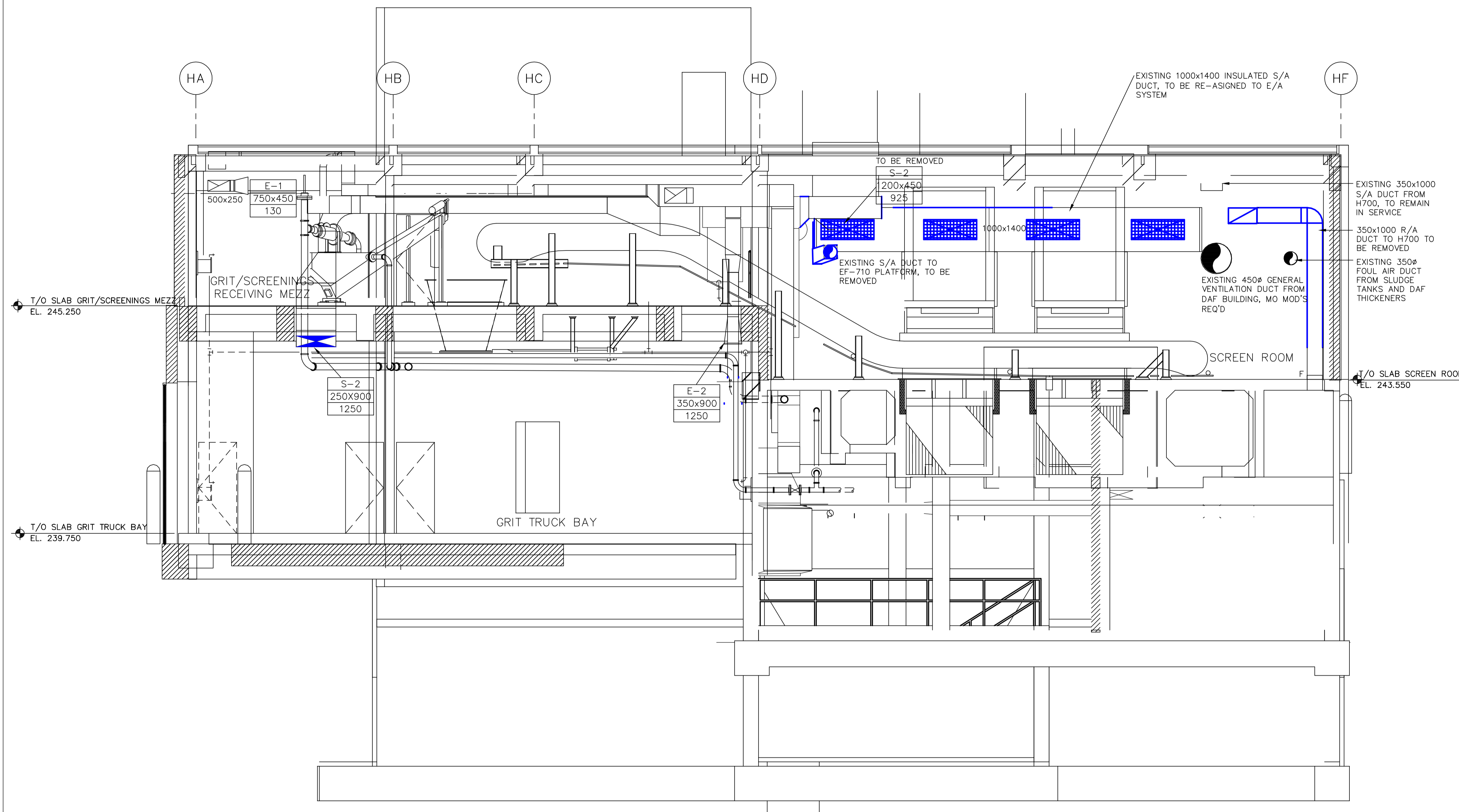
A AREA H - VENTILATION - SECTION AT GRID LINE H3 HM1.9 SCALE 1:50
