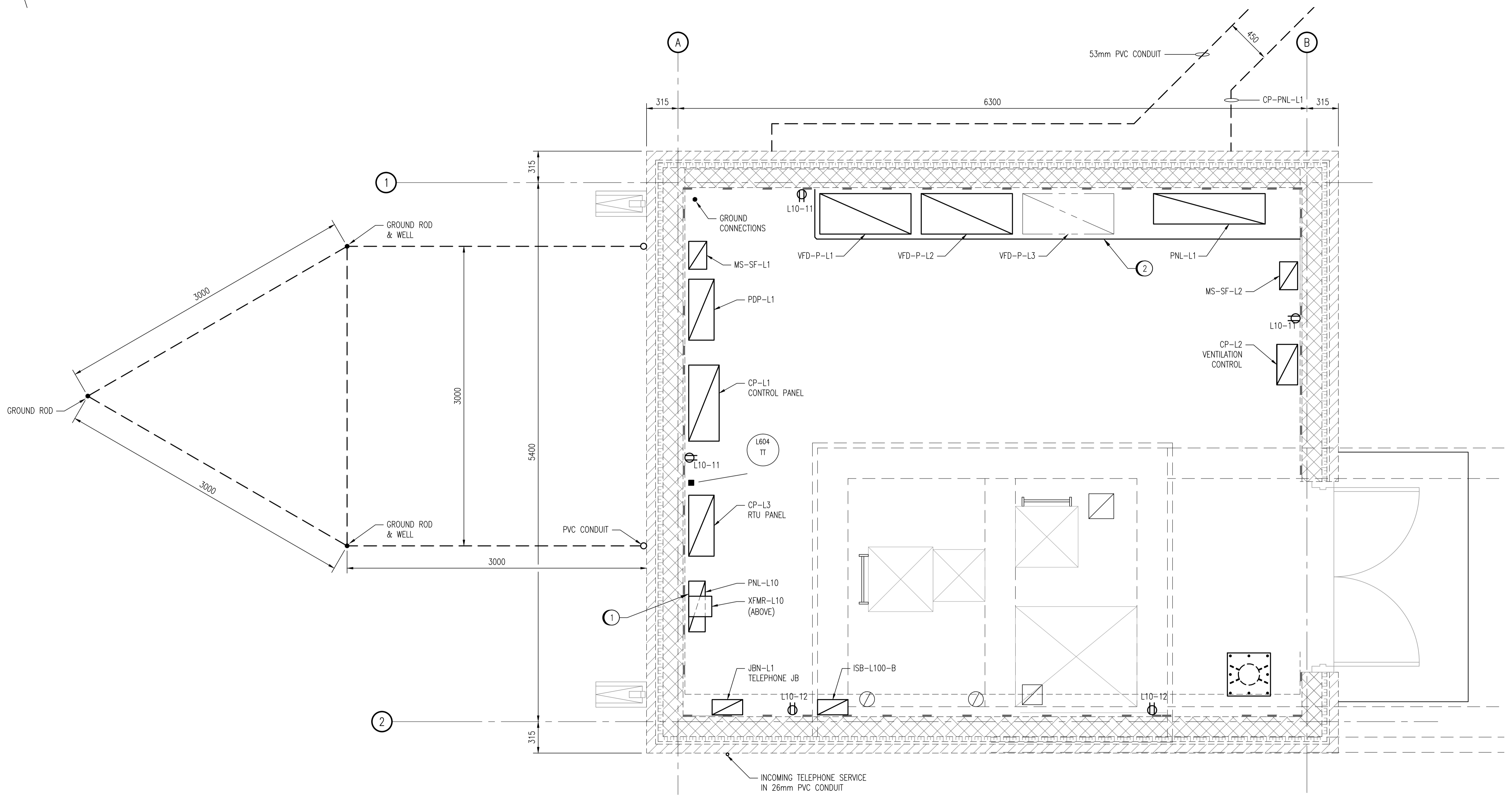
MAIN FLOOR PLAN SCALE: 1 : 20
