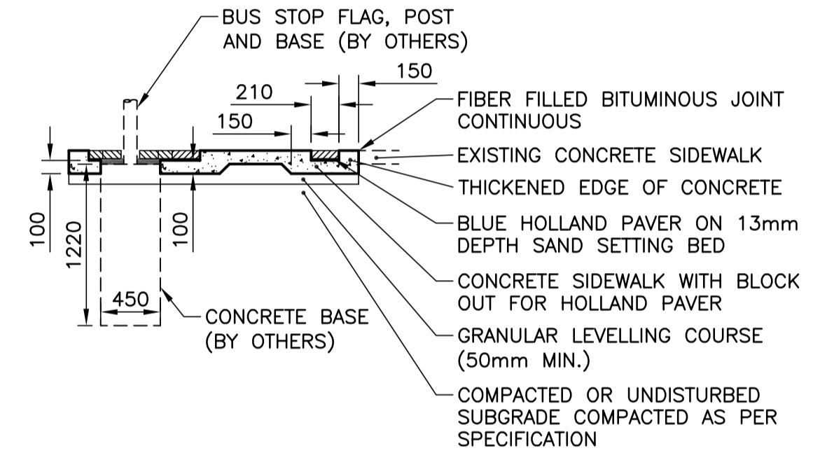
BUS PAD DETAIL SCALE: 1:40
