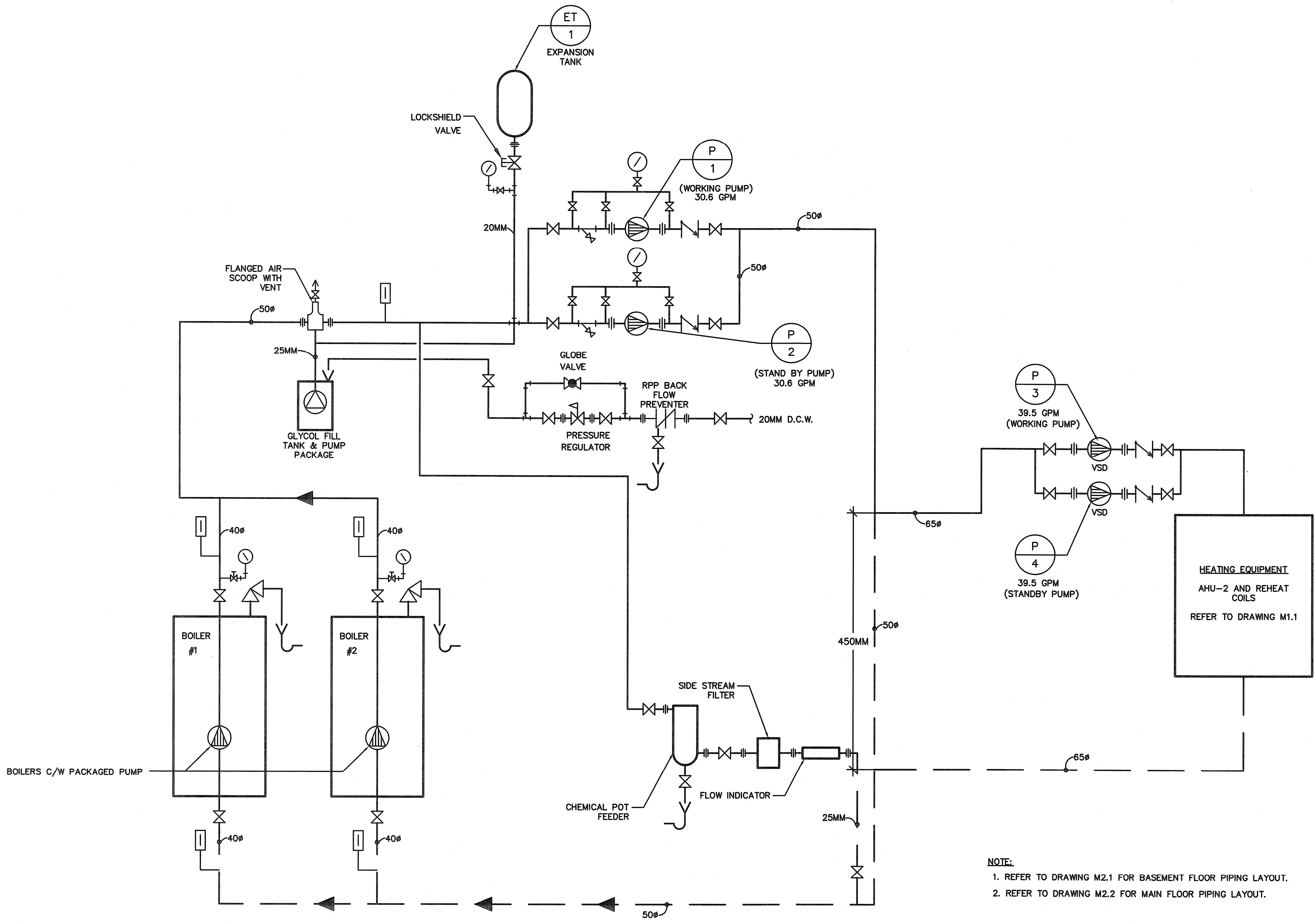
1 HEATING PIPING SCHEMATIC M9.1 SCALE: NTS
