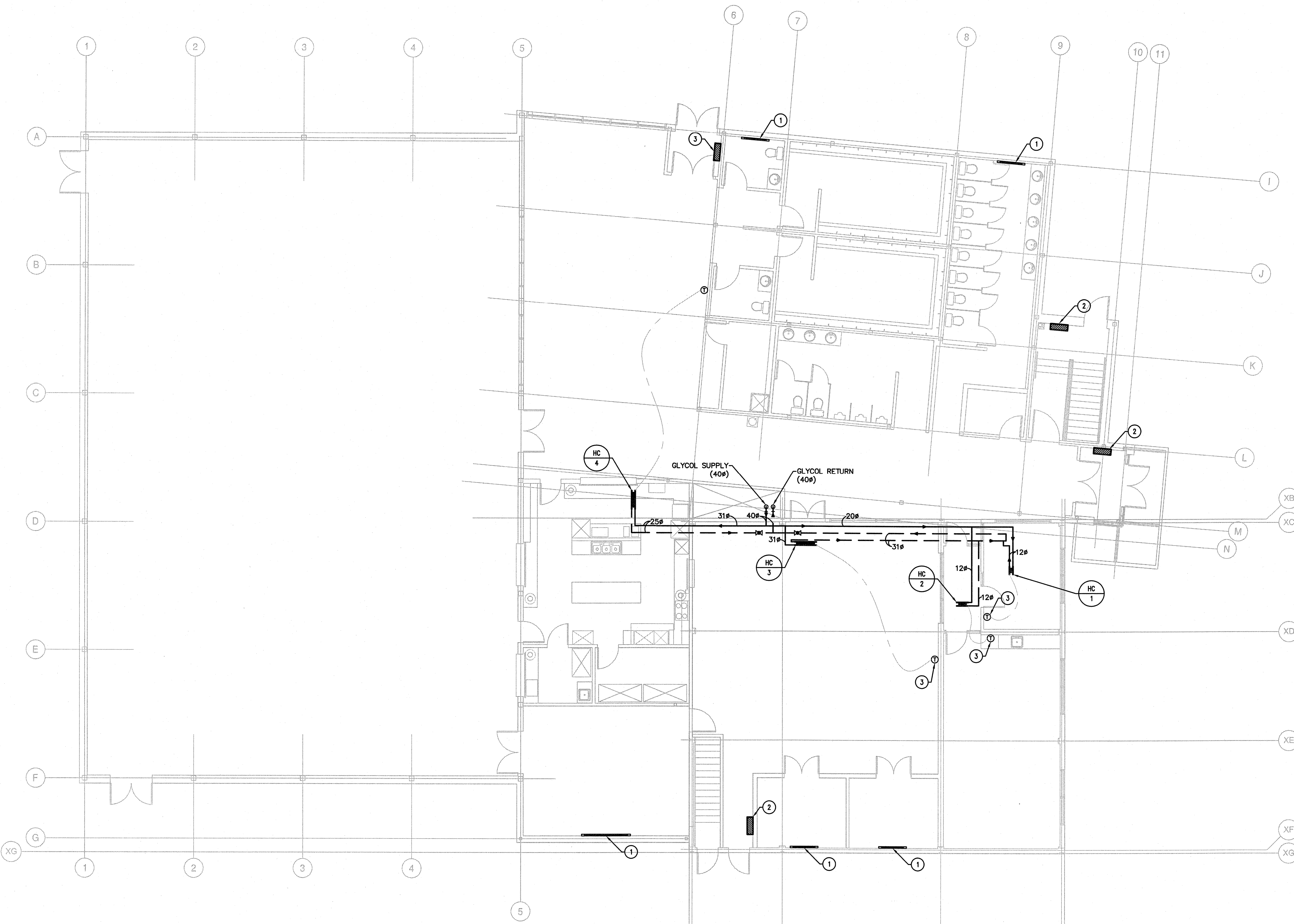
1 MAIN FLOOR PLAN- HEATING LAYOUT M4.2 SCALE: 1:100
