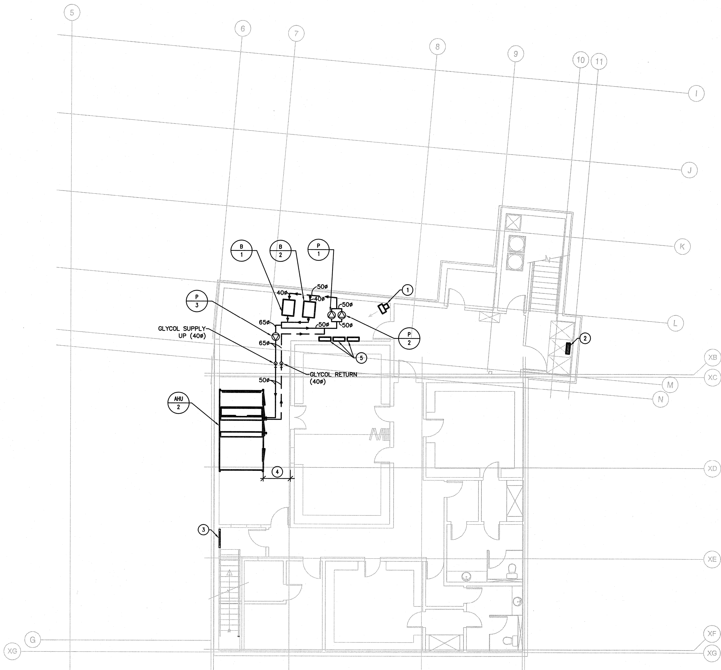
1 BASEMENT PLAN- HEATING LAYOUT M4.1 SCALE: 1:100
