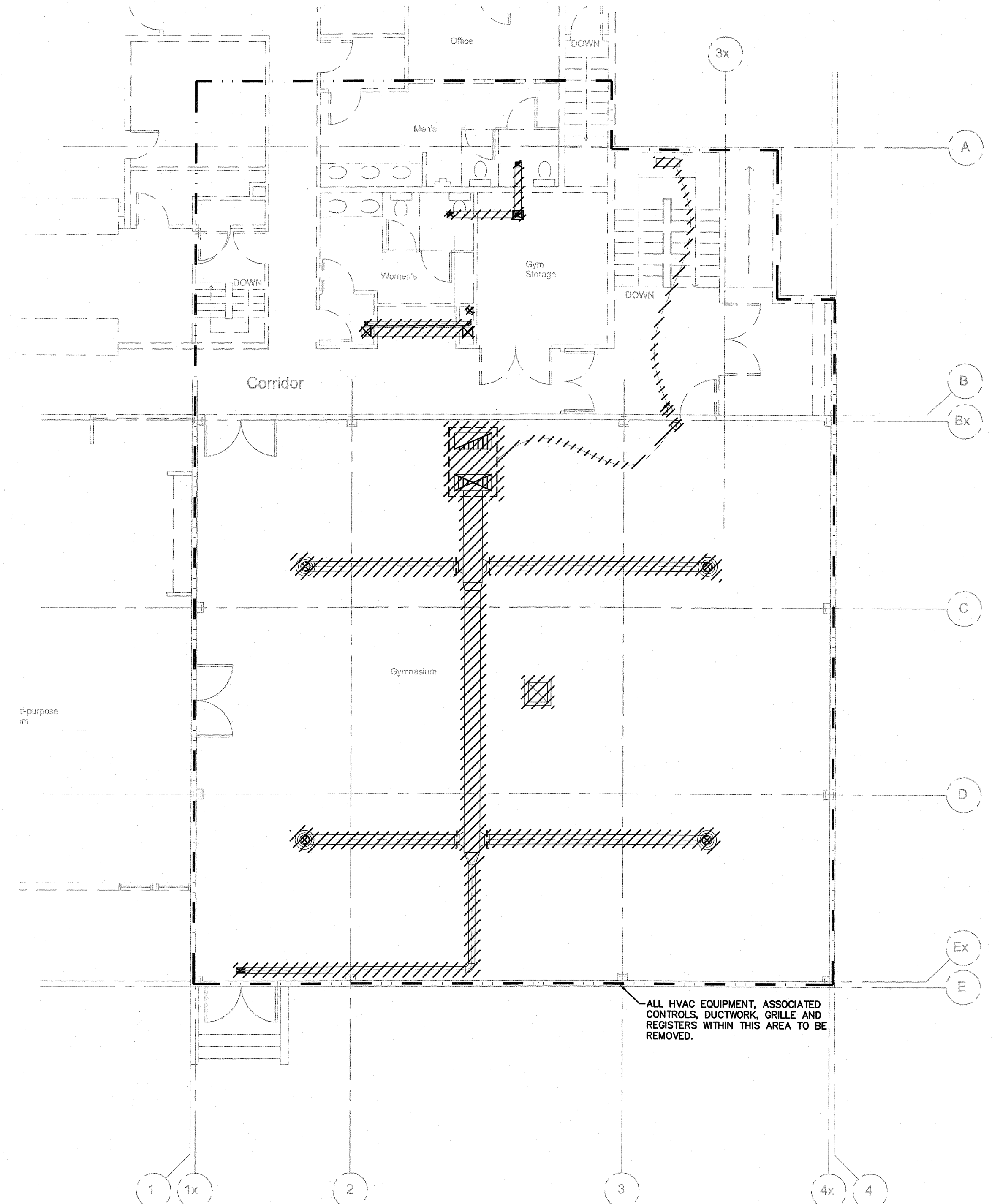
2 MAIN FLOOR PLAN- HVAC DEMOLITION LAYOUT M1.1 SCALE: 1:100
