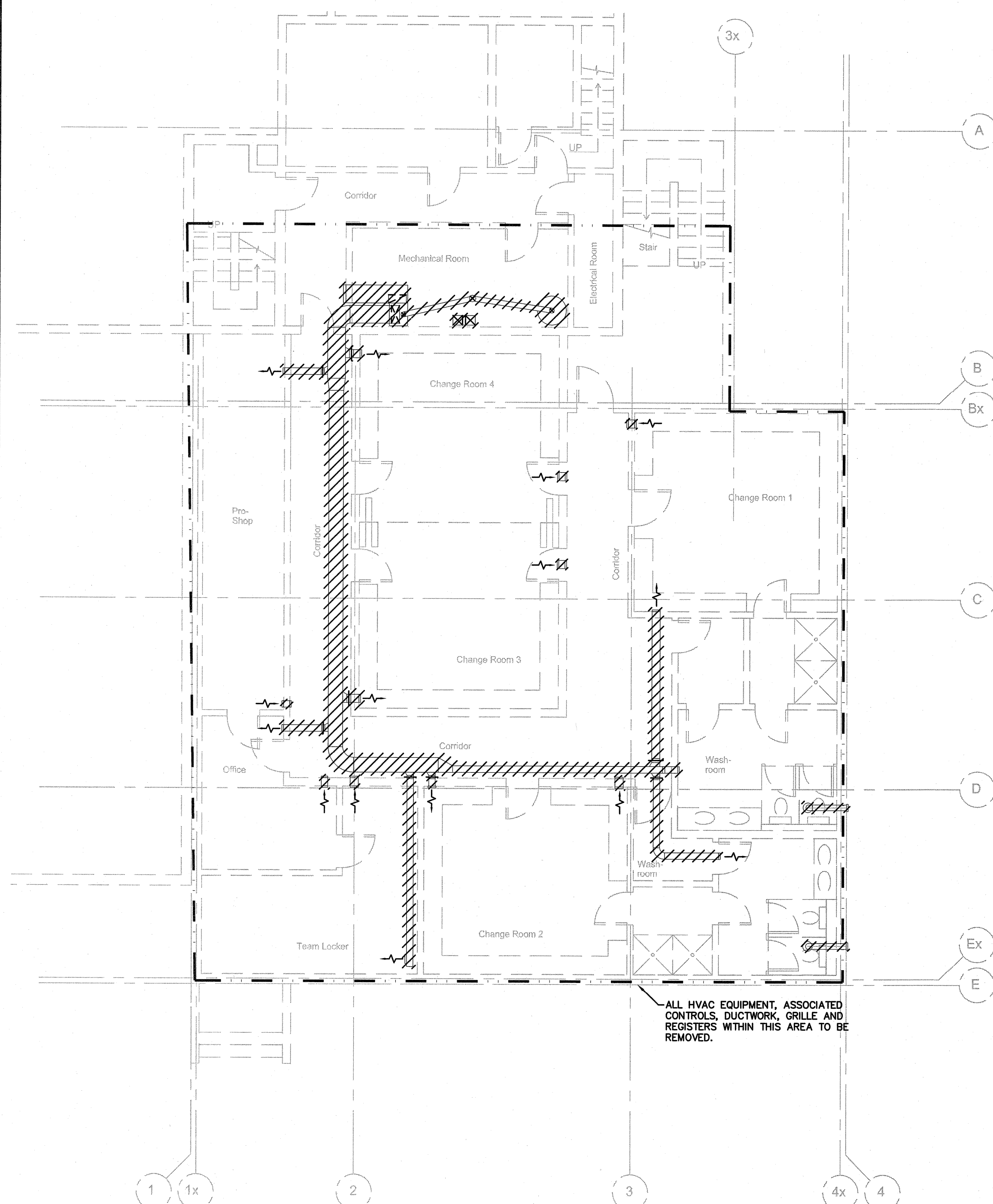
1 BASEMENT PLAN- HVAC DEMOLITION LAYOUT M1.1 SCALE: 1:100
