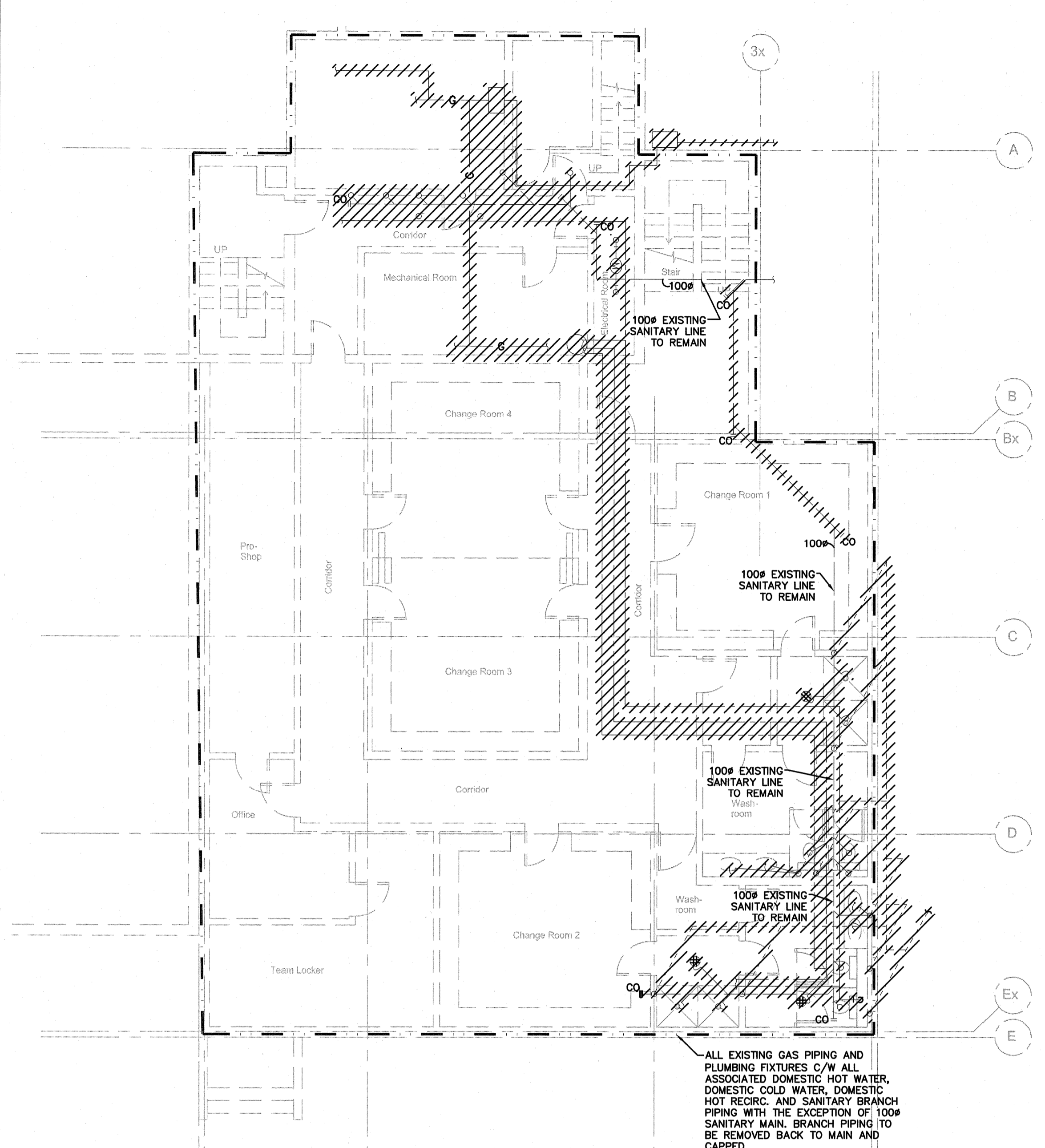
1 BASEMENT PLAN- PLUMBING DEMOLITION LAYOUT M1.1 SCALE: 1:100
