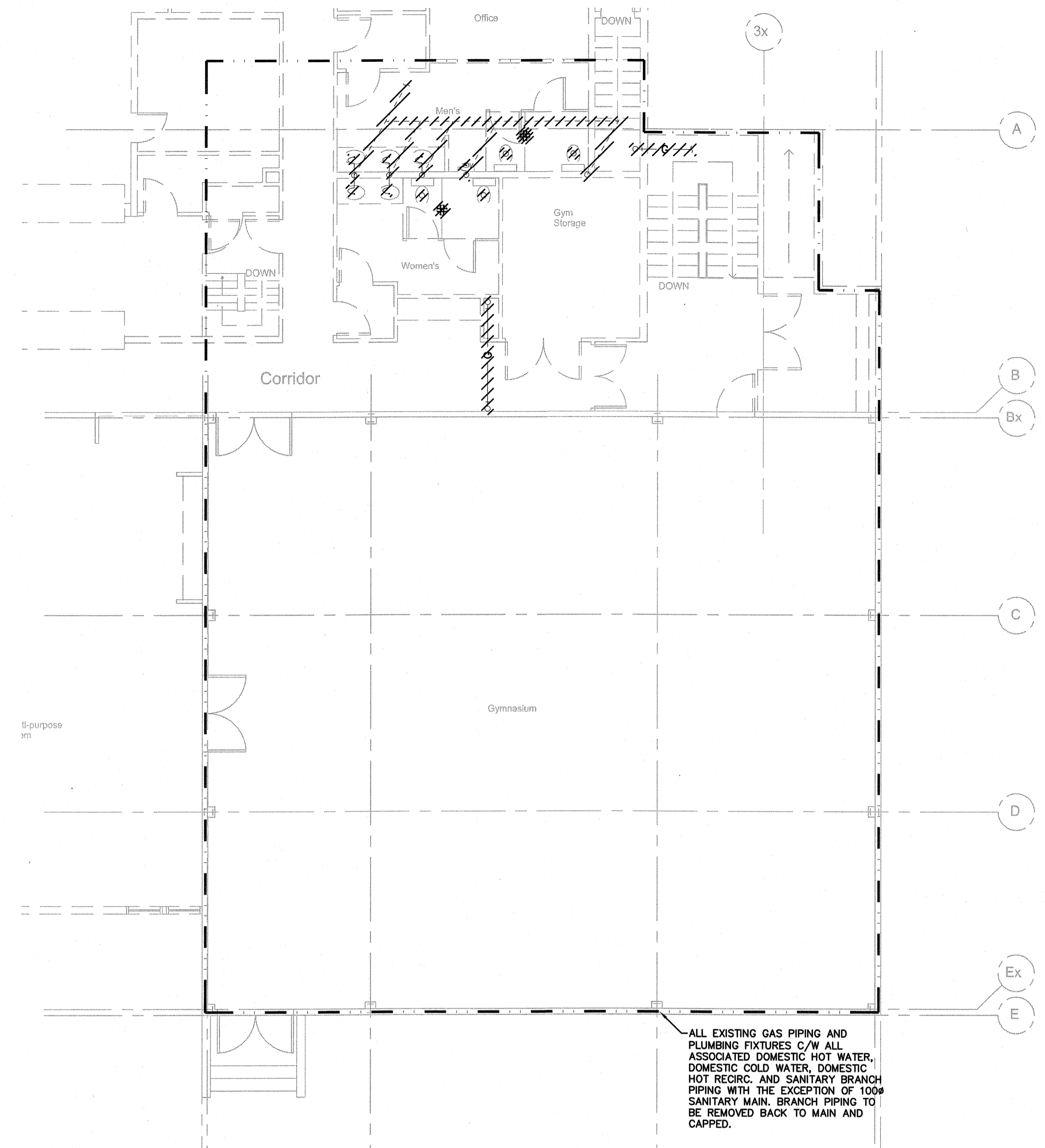
2 MAIN FLOOR PLAN- PLUMBING DEMOLITION LAYOUT M1.1 SCALE: 1:100
