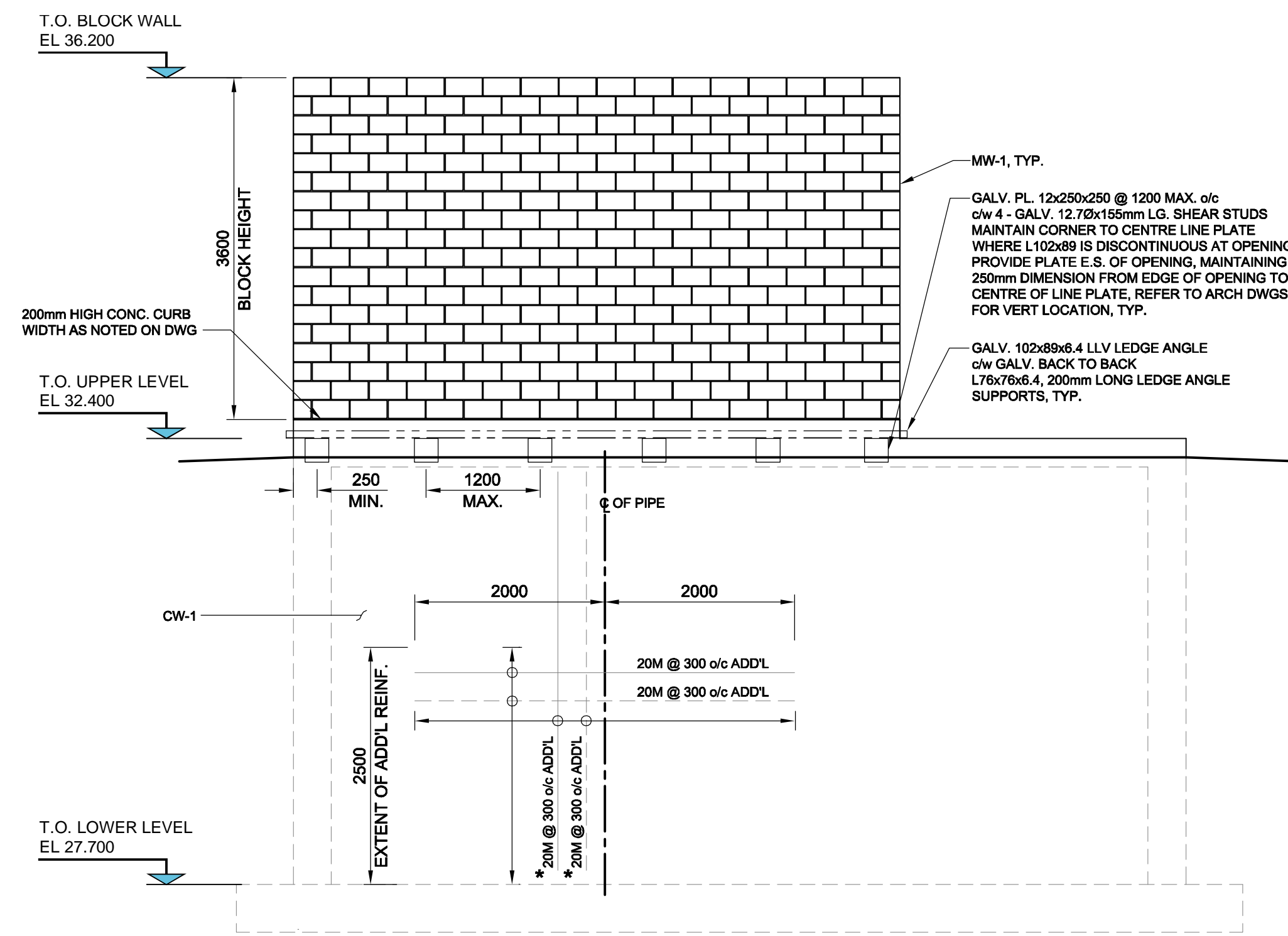
SOUTH ELEVATION
