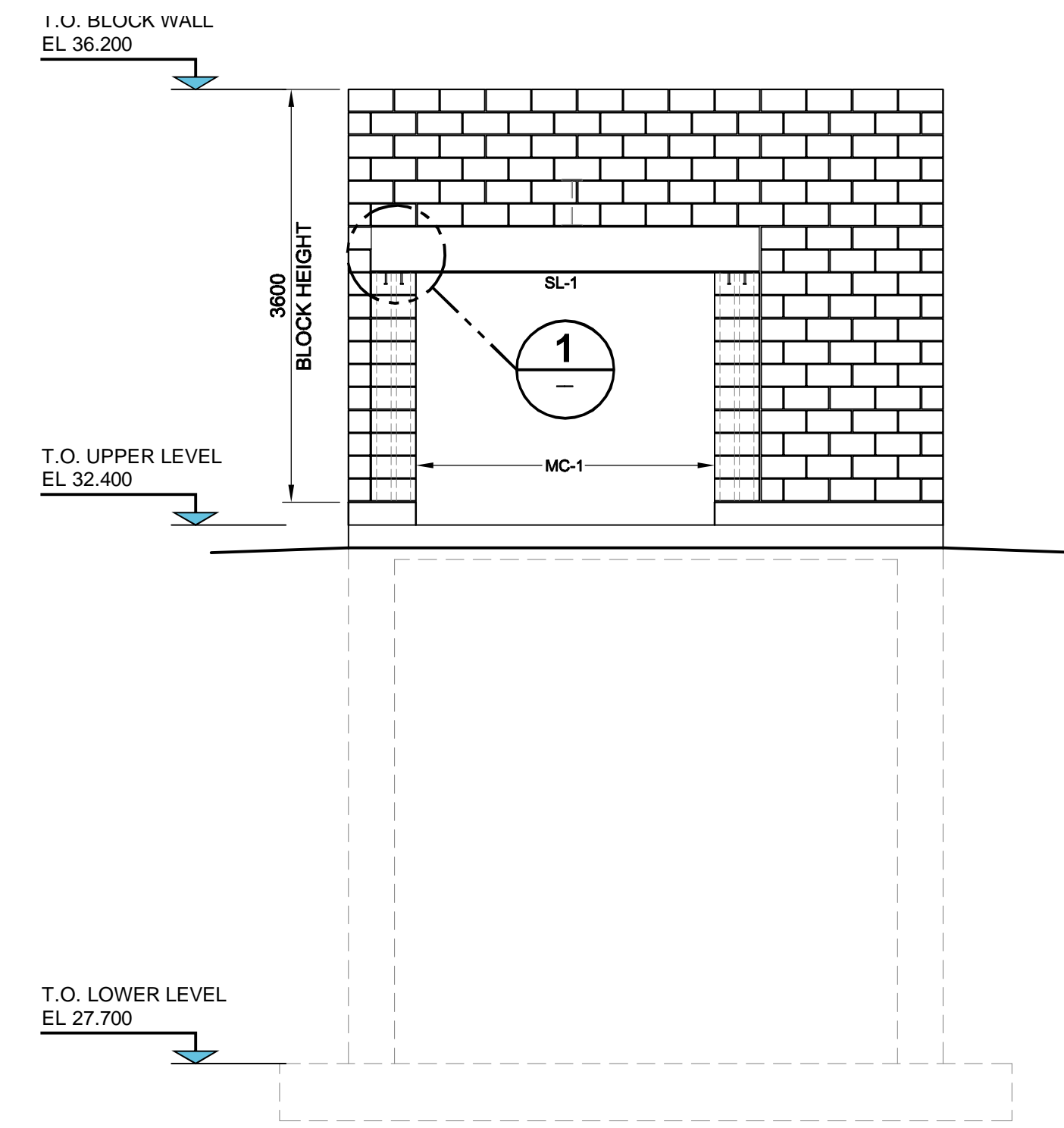
EAST ELEVATION
