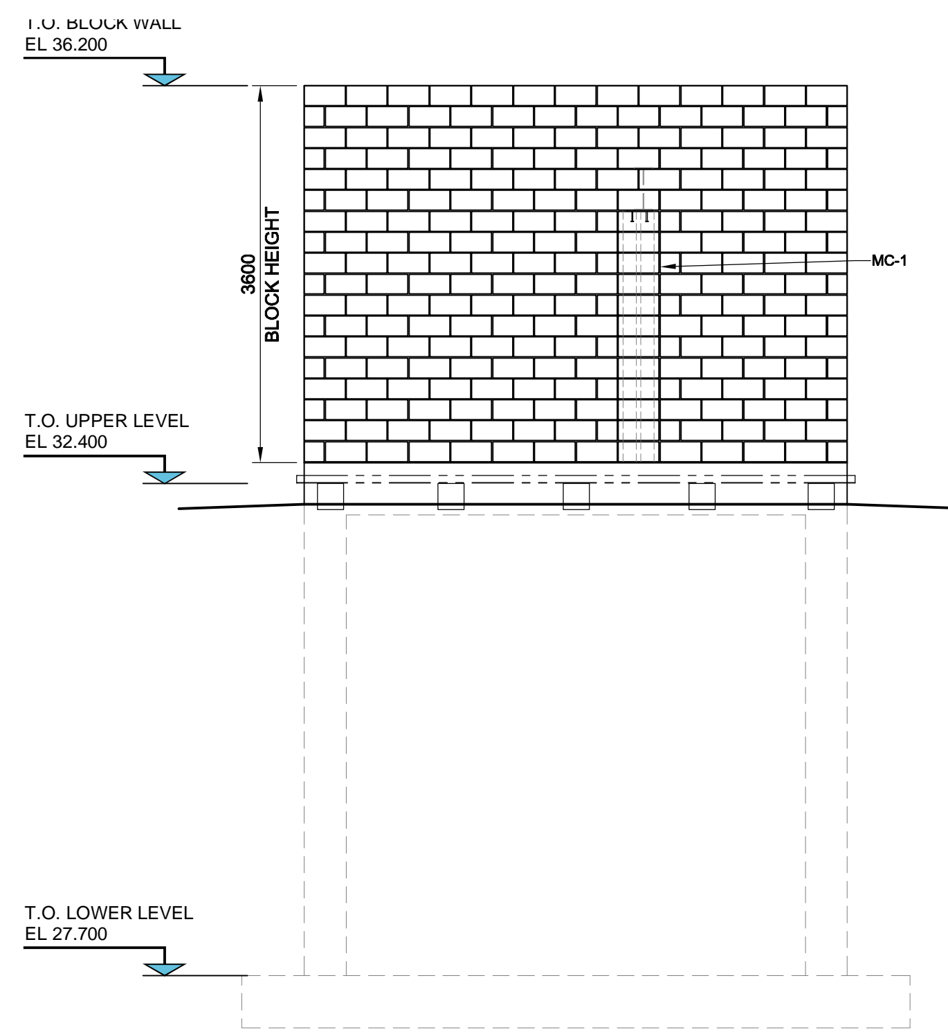
WEST ELEVATION
