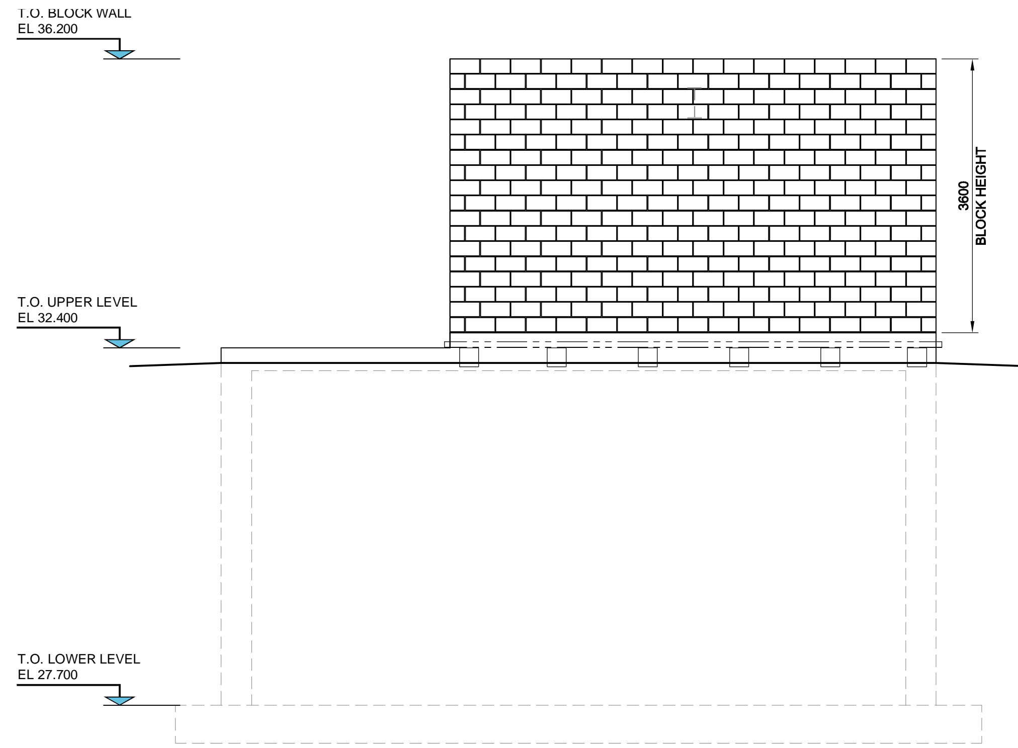
NORTH ELEVATION
