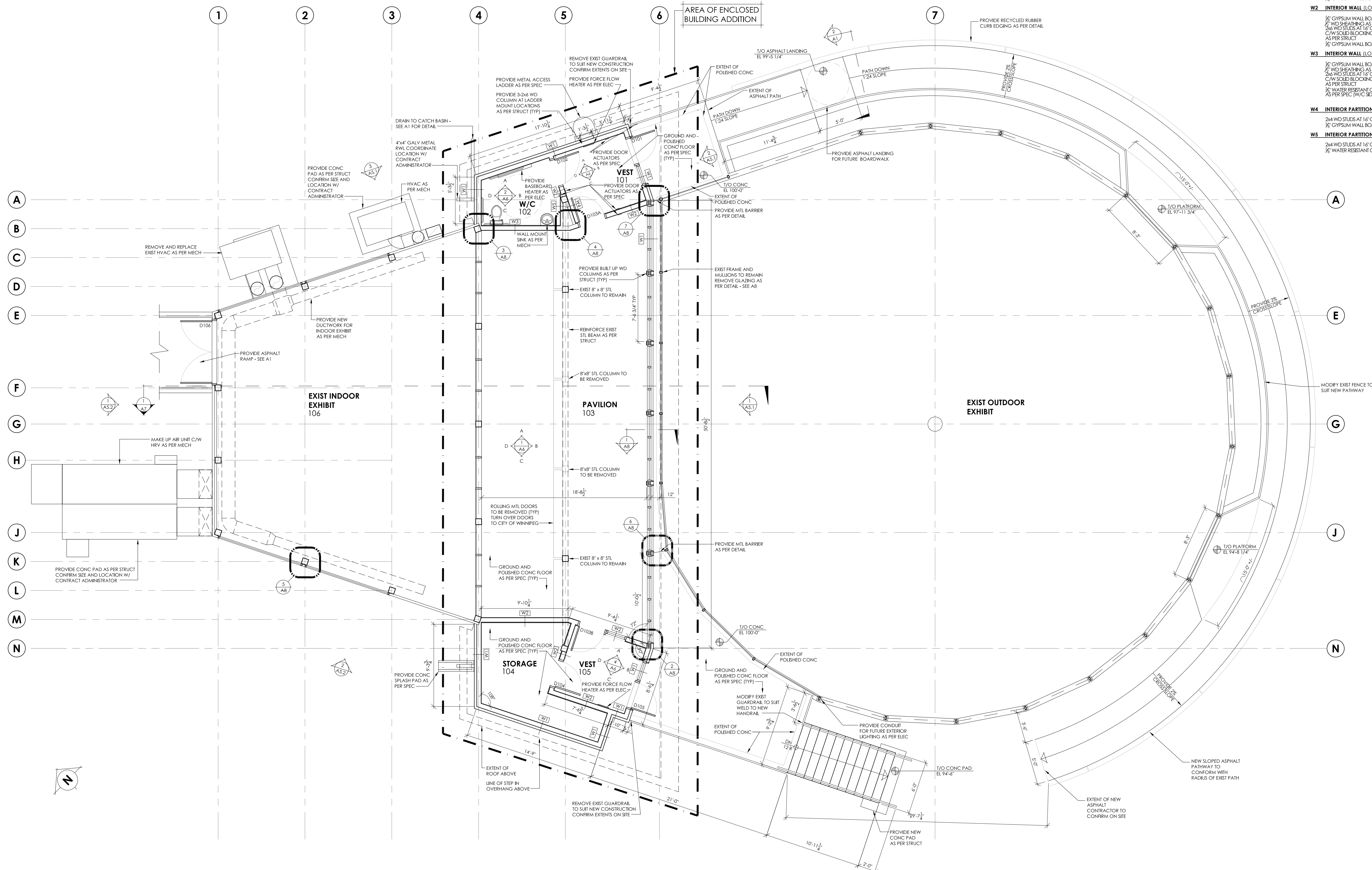
1 MAIN FLOOR PLAN 3/16" = 1'-0"
