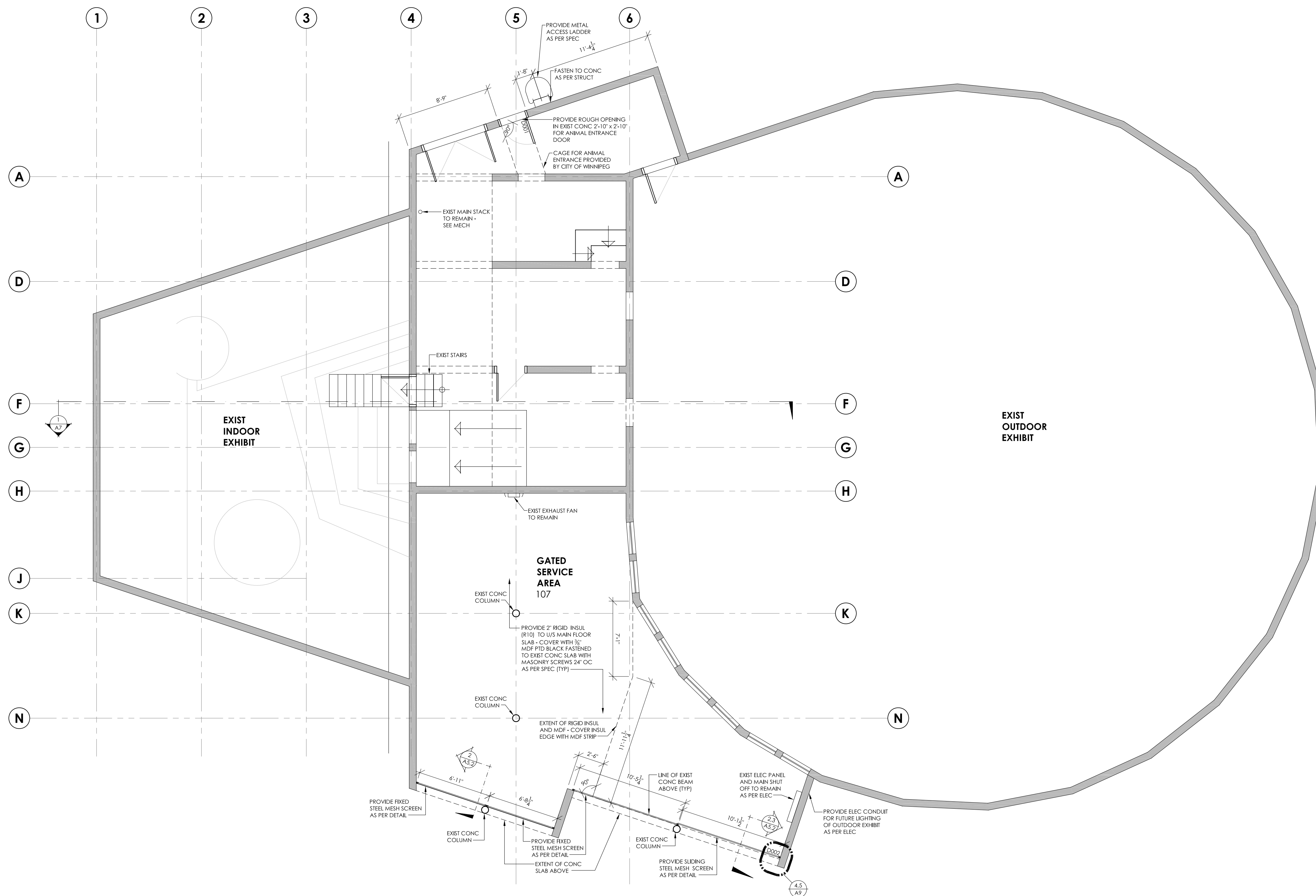
1 BASEMENT FLOOR PLAN 3/16" = 1'-0"
