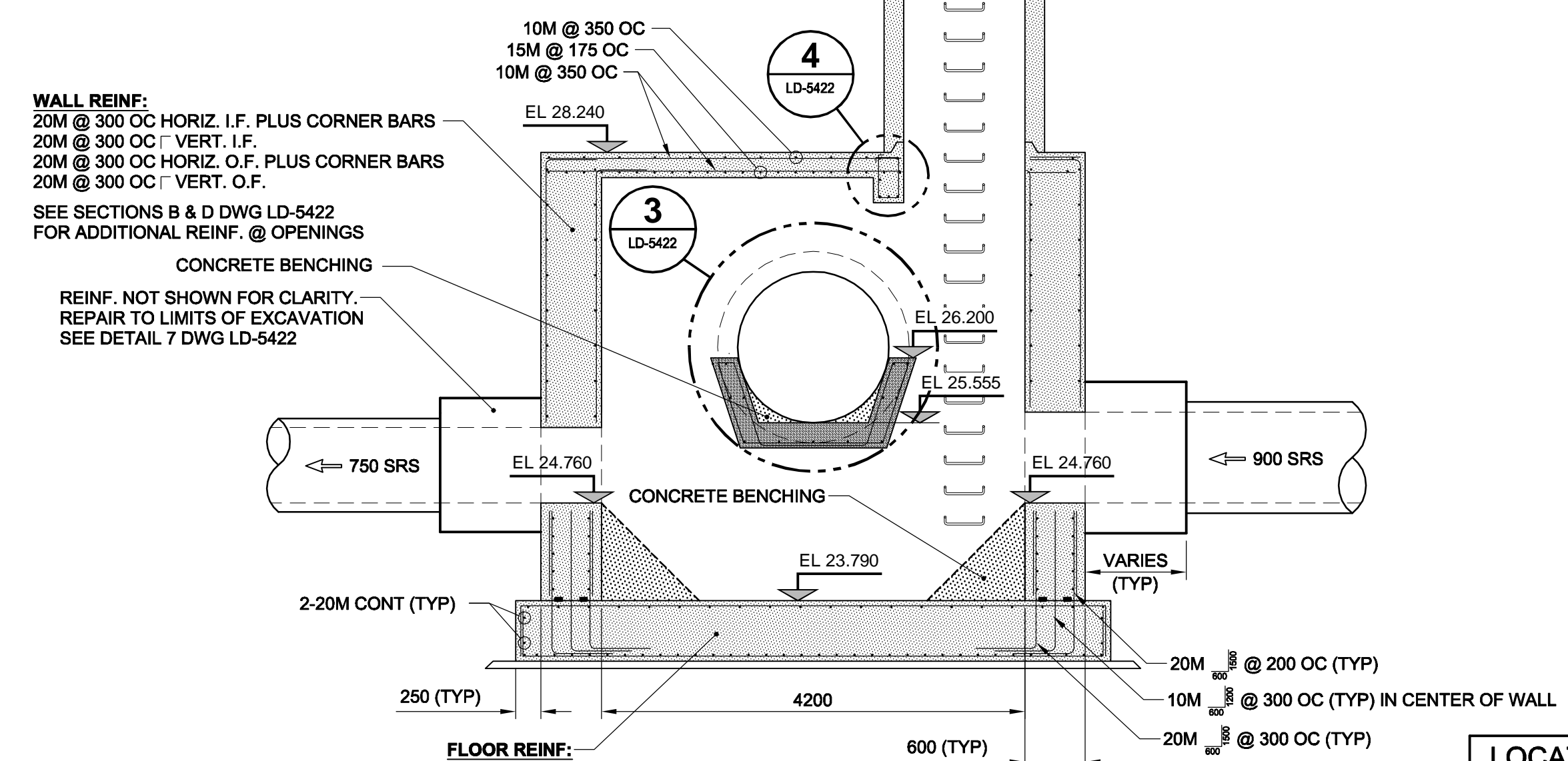
SECTION A
