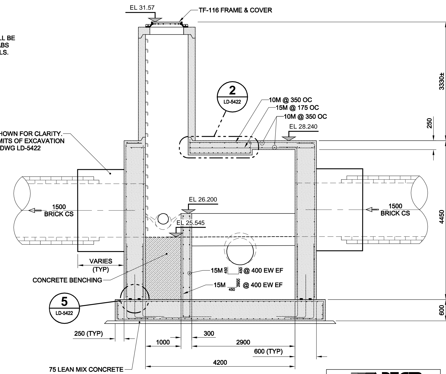
SECTION B
