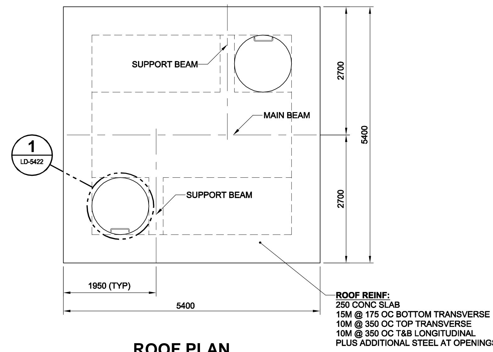
ROOF PLAN
