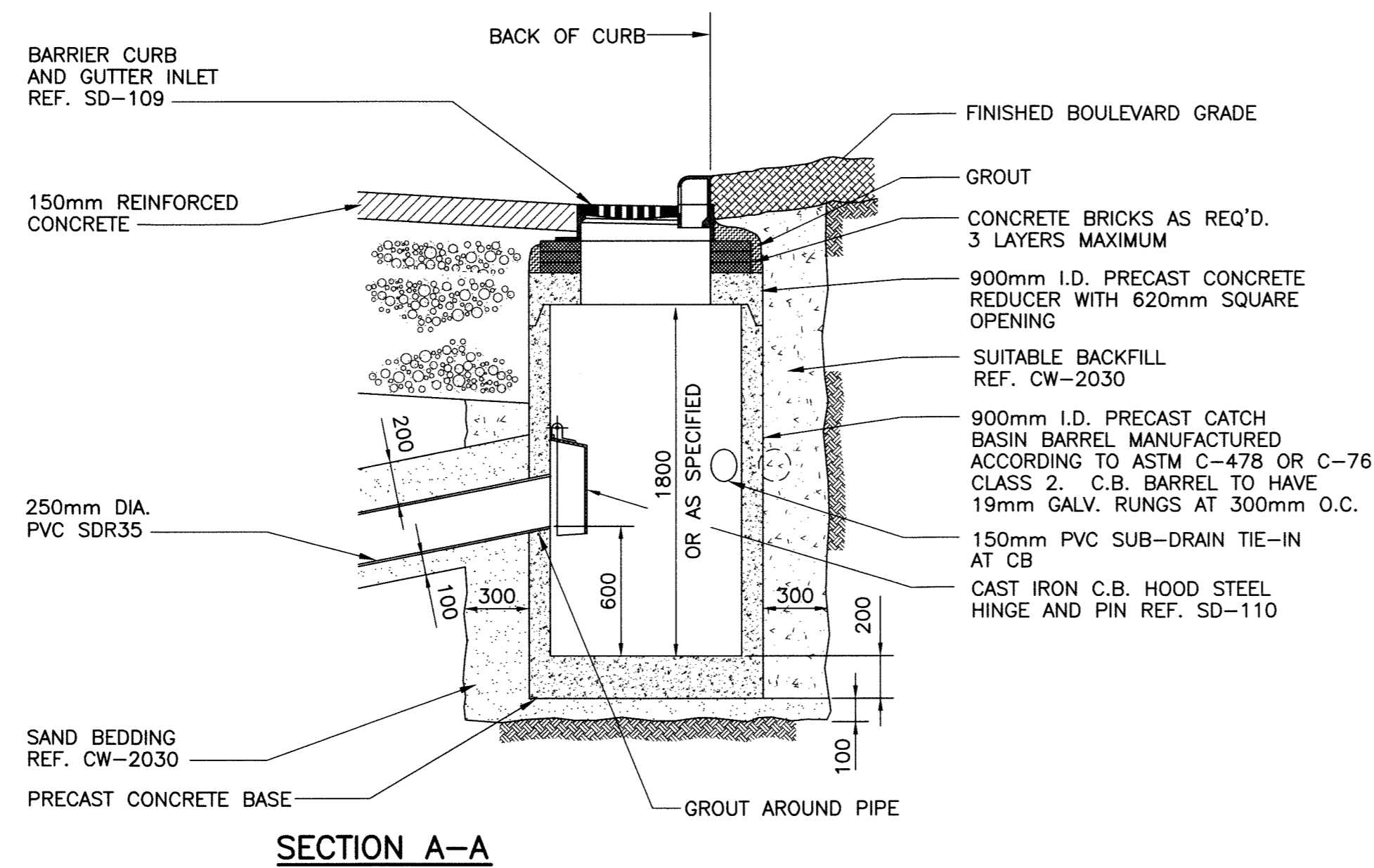
CATCH BASIN DETAIL SCALE: 1:25
